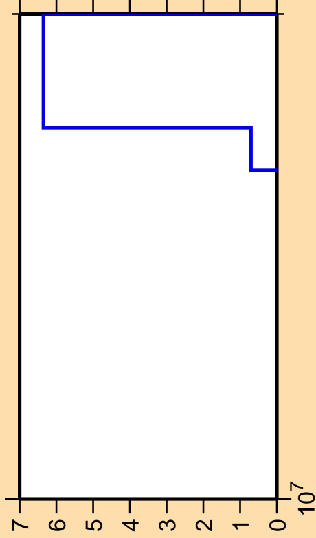
\Delta\sigma/\sigma vs. E for ^{152}\text{Eu} (mt 45)
