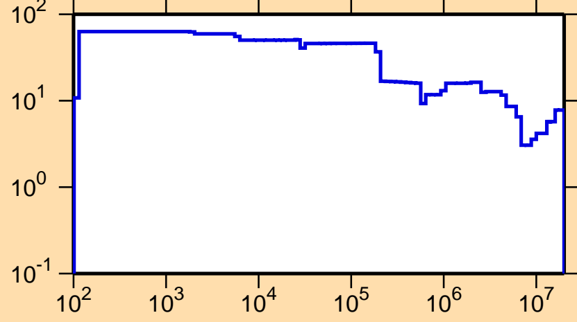
\Delta\sigma/\sigma vs. E for ^{152}\text{Eu}(n,\text{tot.})
