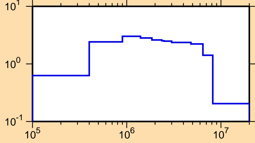
\sigma vs. E for ^{152}\text{Eu}(n,n\text{cont.})
