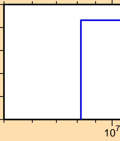
\sigma vs. E for ^{152}\text{Eu}(n,nd)
