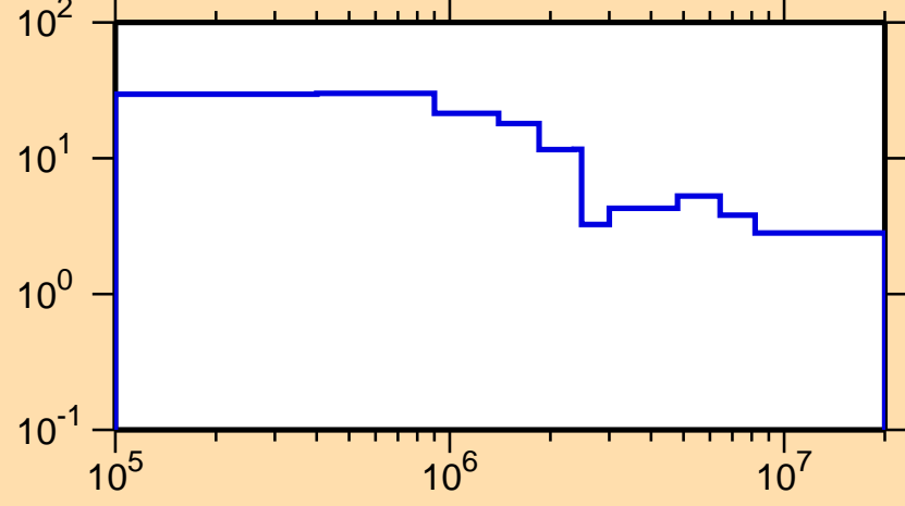
\Delta\sigma/\sigma vs. E for ^{152}\text{Eu}(n,n\text{nonel.})
