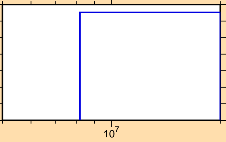
\sigma vs. E for ^{152}\text{Eu}(n,2n\alpha)
