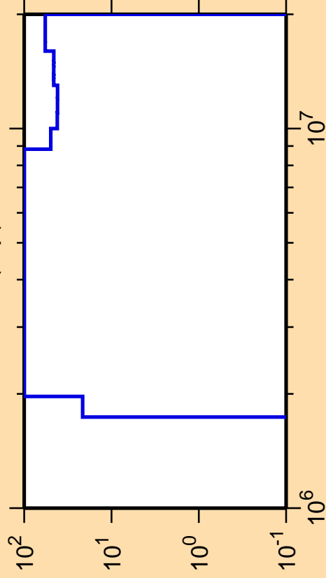
\Delta\sigma/\sigma vs. E for ^{153}\text{Eu}(n,p)
