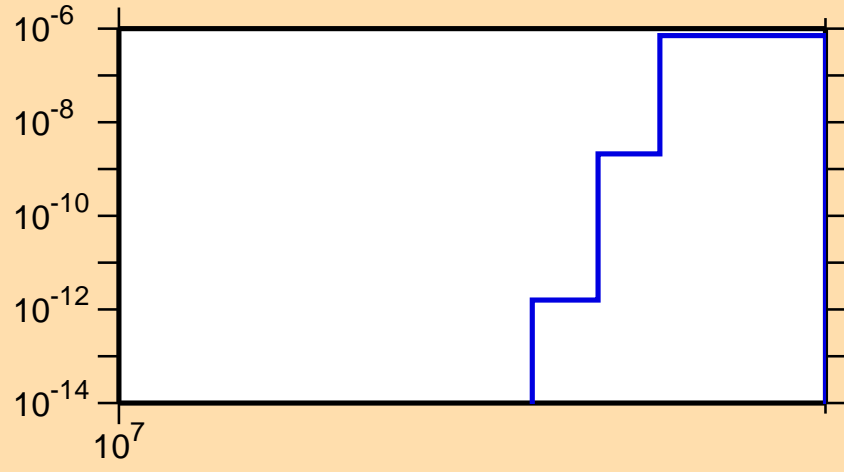
\sigma vs. E for ^{153}\text{Eu}(n,2np)
