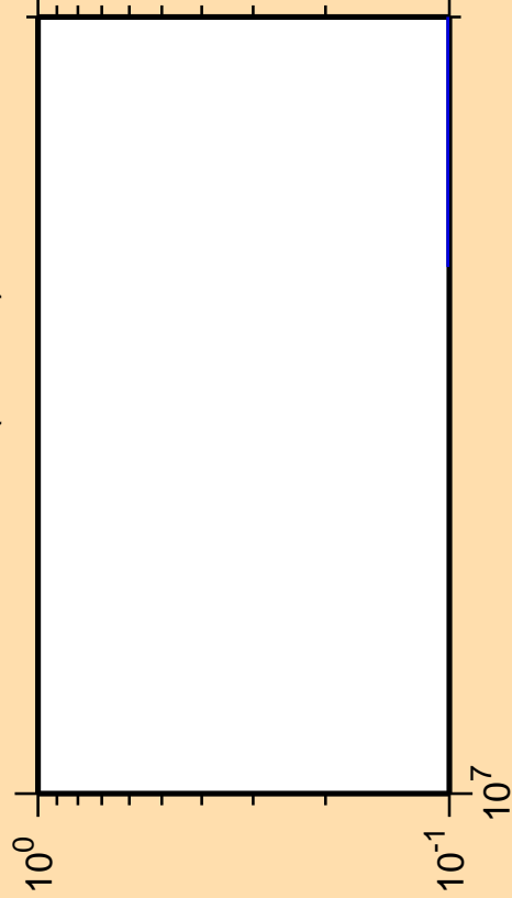
\Delta\sigma/\sigma vs. E for ^{153}\text{Eu}(n,3n\alpha)
