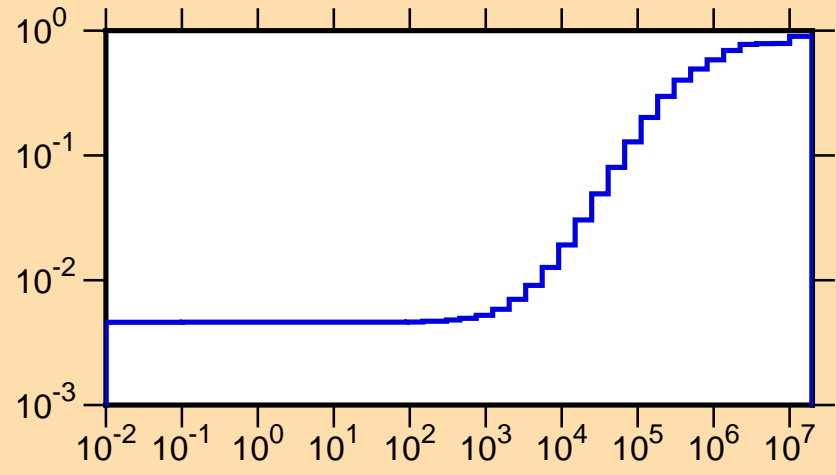
\mu vs. E for ^{153}\text{Eu}(\text{mt251})
