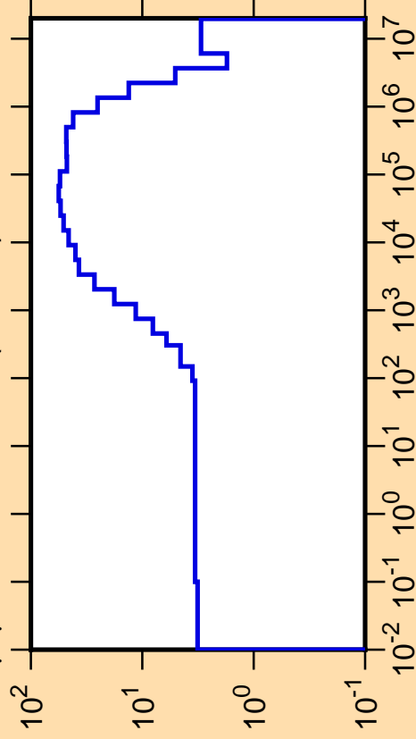
\Delta\mu/\mu vs. E for ^{153}\text{Eu}(\text{mt251})
