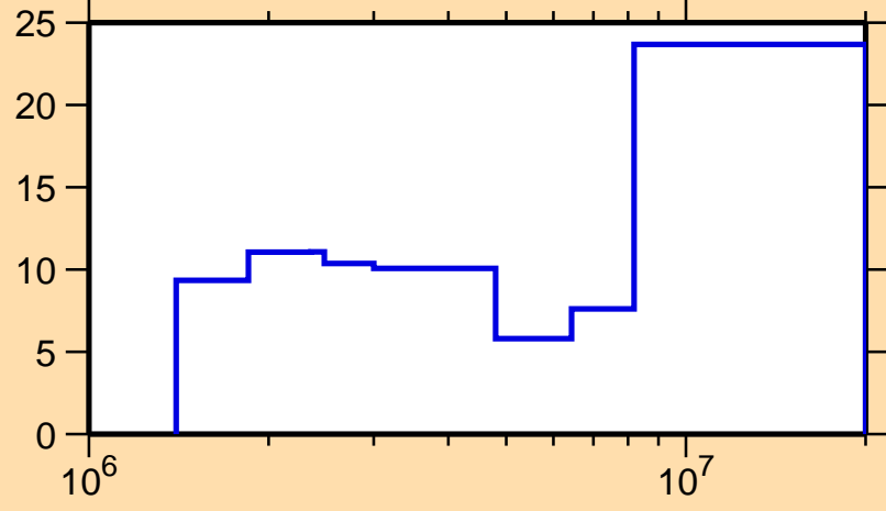
\Delta\sigma/\sigma vs. E for ^{153}\text{Eu}(n,ncont.)
