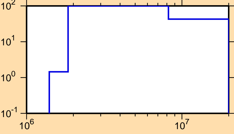
\Delta\sigma/\sigma vs. E for ^{153}\text{Eu}(n,p)
