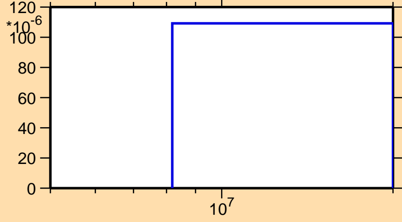
\sigma vs. E for ^{153}\text{Eu}(n,t)
