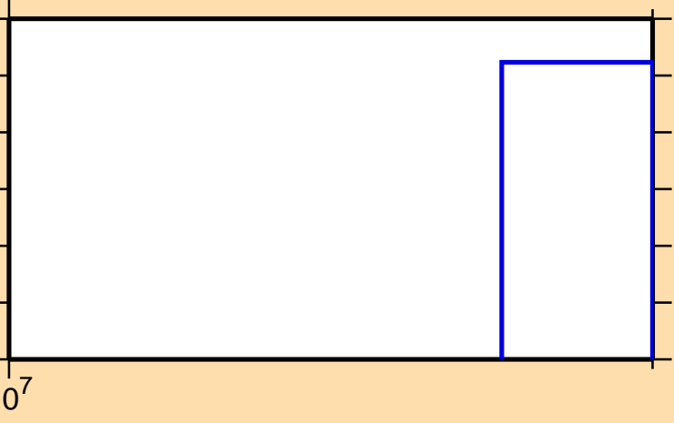
\sigma vs. E for ^{154}\text{Eu} (mt 11)
