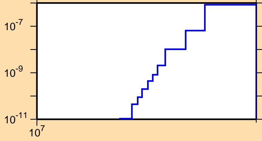
\sigma vs. E for ^{154}\text{Eu}(n,2n\alpha)
