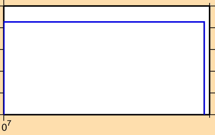
\sigma vs. E for ^{154}\text{Eu}(n,3n)
