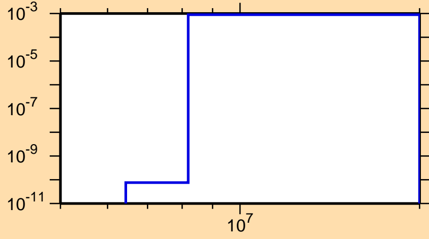
\sigma vs. E for ^{154}\text{Eu}(n,d)
