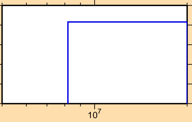
\sigma vs. E for ^{154}\text{Eu}(n,\text{nd})
