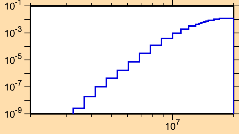
\sigma vs. E for ^{155}\text{Eu}(n,p)
