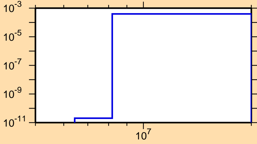
\sigma vs. E for ^{155}\text{Eu}(n,d)
