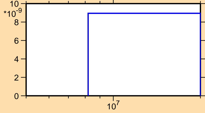
\sigma vs. E for ^{155}\text{Eu}(n,\text{nd})
