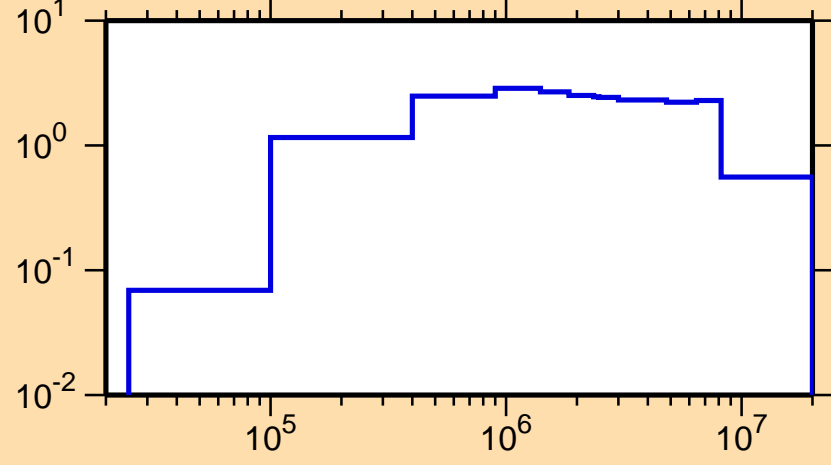
\sigma vs. E for ^{155}\text{Eu}(n,\text{inel.})
