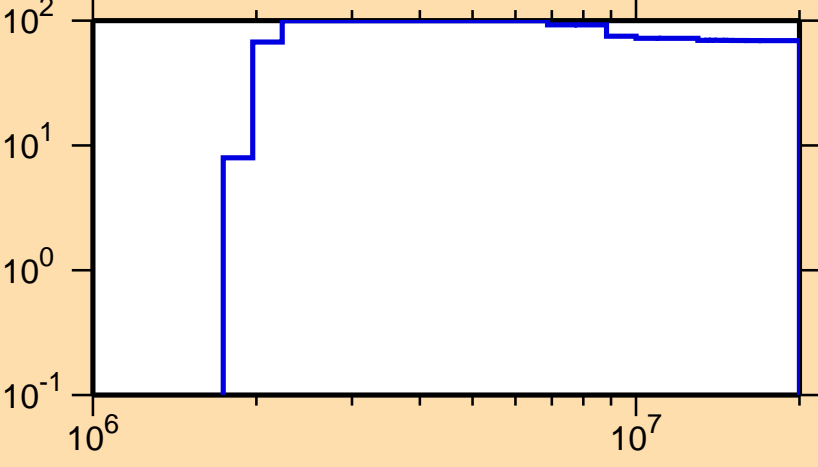
\Delta\sigma/\sigma vs. E for ^{156}\text{Eu}(n,p)
