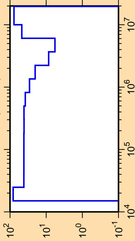
\Delta\sigma/\sigma vs. E for ^{156}\text{Eu}(n,\text{inel.})
