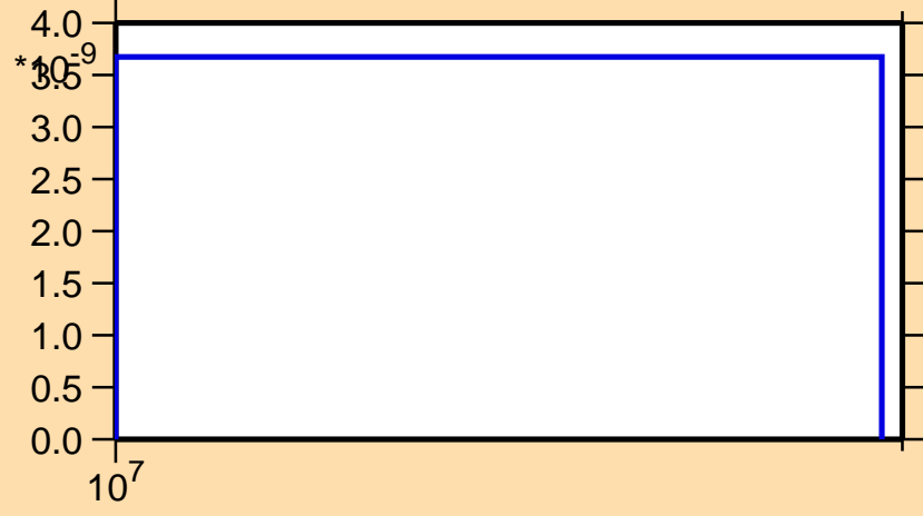
\sigma vs. E for ^{156}\text{Eu}(n,nt)
