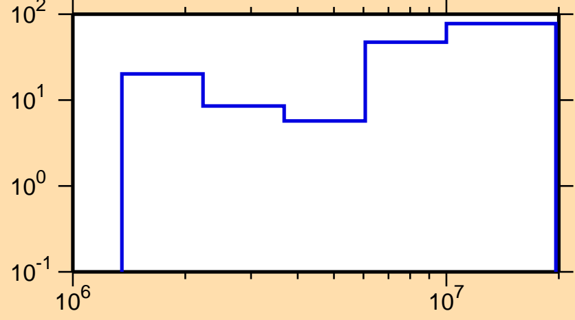
\Delta\sigma/\sigma vs. E for ^{156}\text{Eu}(n,\text{inel.})
