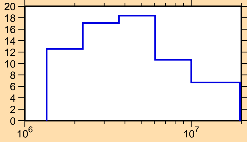
\Delta\sigma/\sigma vs. E for ^{156}\text{Eu}(n,el.)
