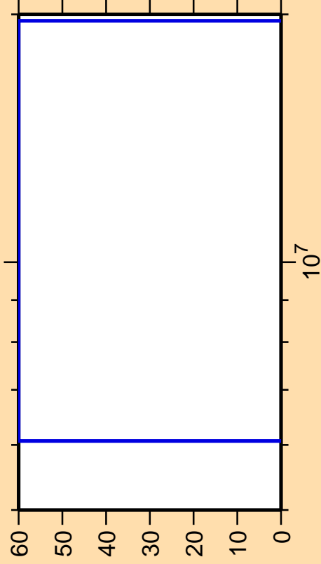
\Delta\sigma/\sigma vs. E for ^{156}\text{Eu}(n,\gamma)
