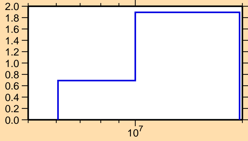
\sigma vs. E for ^{156}\text{Eu}(n,2n)
