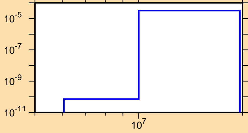
\sigma vs. E for ^{156}\text{Eu}(n,n\alpha)
