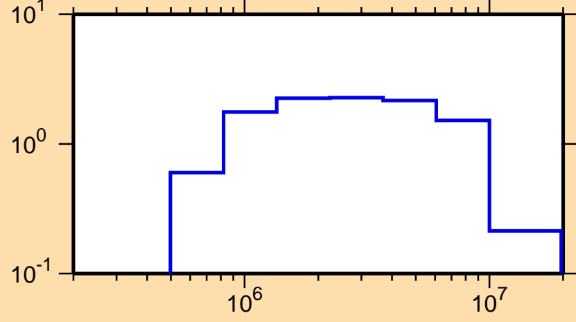
\sigma vs. E for ^{156}\text{Eu}(n,n\text{cont.})
