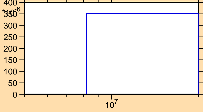
\sigma vs. E for ^{156}\text{Eu}(n,np)
