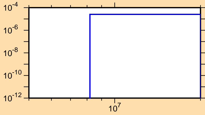
\sigma vs. E for ^{156}\text{Eu}(n,n\alpha)
