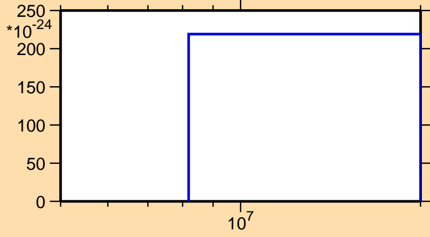
\sigma vs. E for ^{156}\text{Eu}(\text{mt 11})
