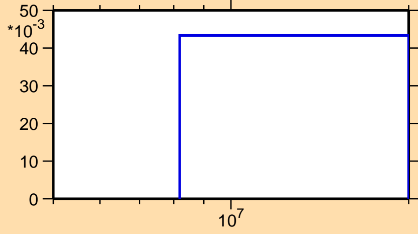
\sigma vs. E for ^{156}\text{Eu}(n,3n)
