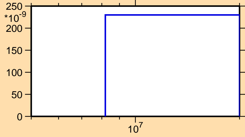
\sigma vs. E for ^{156}\text{Eu}(n,nd)
