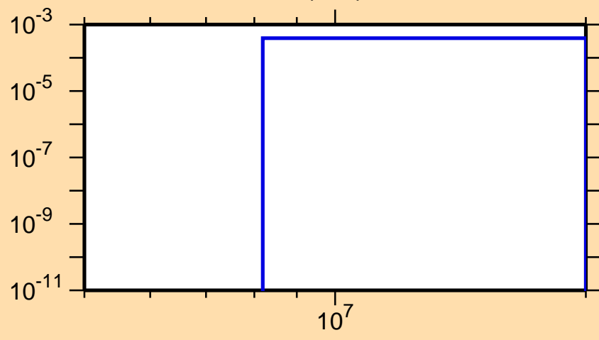
\sigma vs. E for ^{156}\text{Eu}(n,d)
