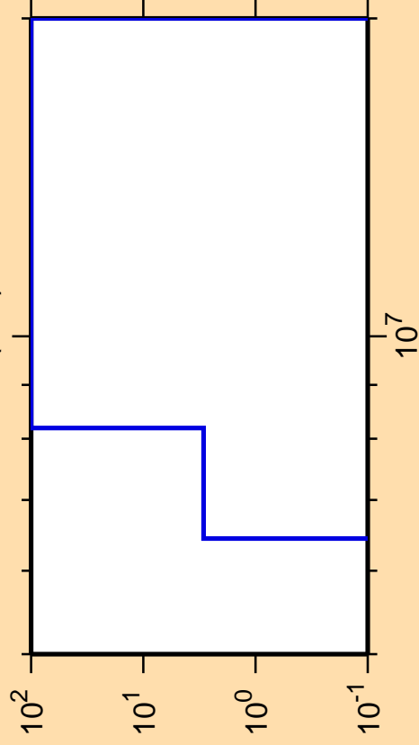
\Delta\sigma/\sigma vs. E for ^{156}\text{Eu}(n,d)
