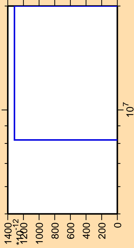
\Delta\sigma/\sigma vs. E for ^{156}\text{Eu}(\text{mt 11})
