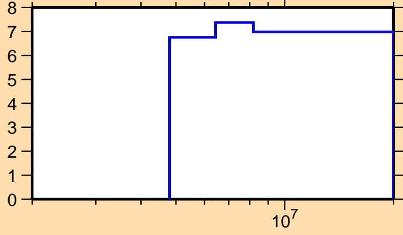
\Delta\sigma/\sigma vs. E for ^{156}\text{Eu}(n,\text{nonel.})
