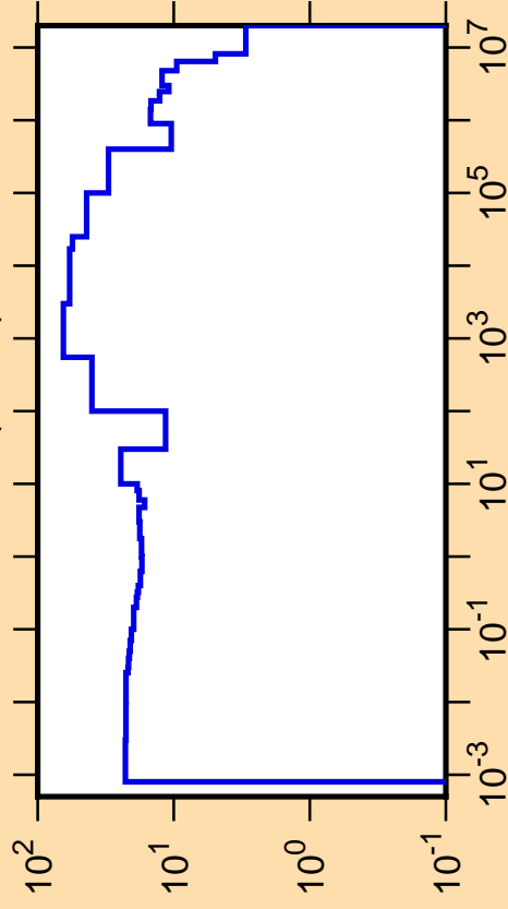
\Delta\sigma/\sigma vs. E for ^{156}\text{Eu}(n,\text{tot.})
