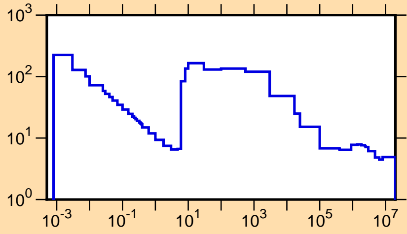
\sigma vs. E for ^{156}\text{Eu}(n,\text{tot.})
