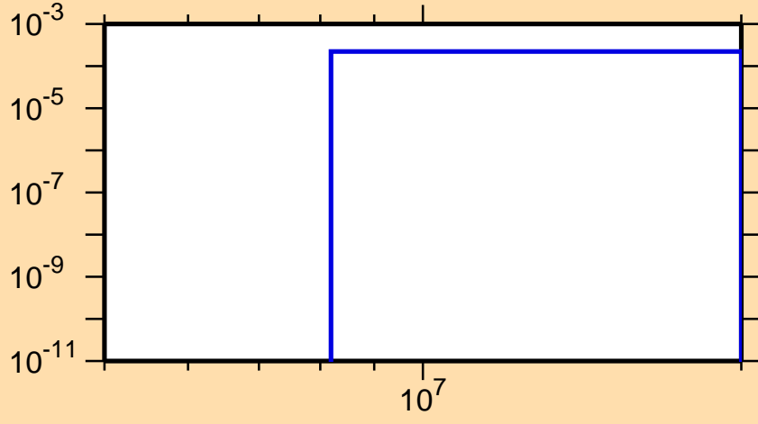
\sigma vs. E for ^{157}\text{Eu}(n,d)
