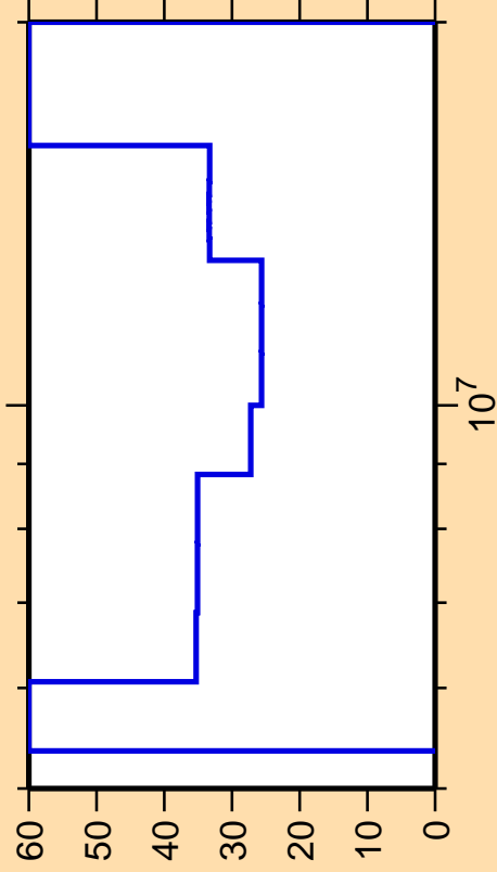
\Delta\sigma/\sigma vs. E for ^{158}\text{Eu}(n,2n)
