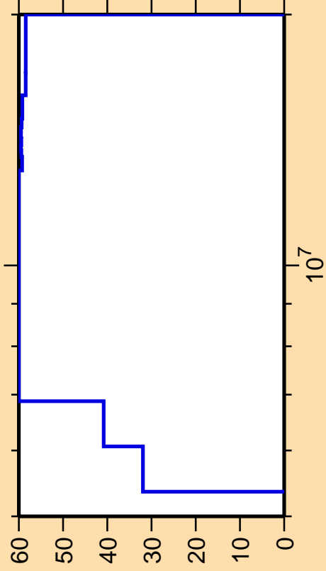
\Delta\sigma/\sigma vs. E for ^{158}\text{Eu}(n,n\text{cont.})
