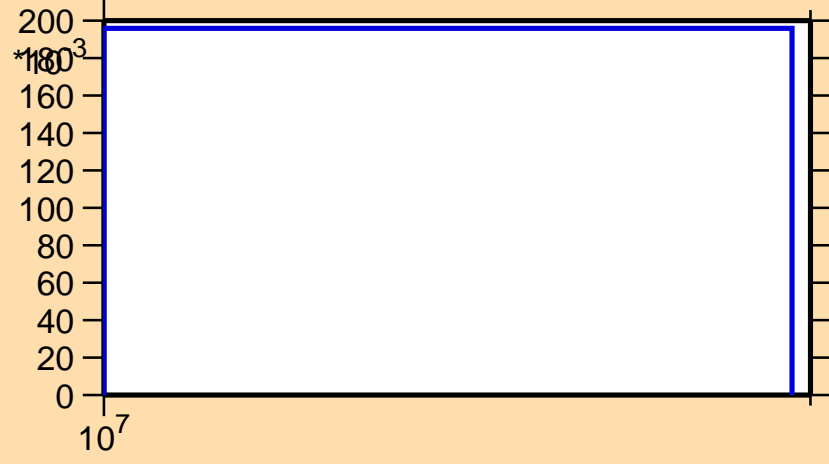
\sigma vs. E for ^{158}\text{Eu}(n,3n)
