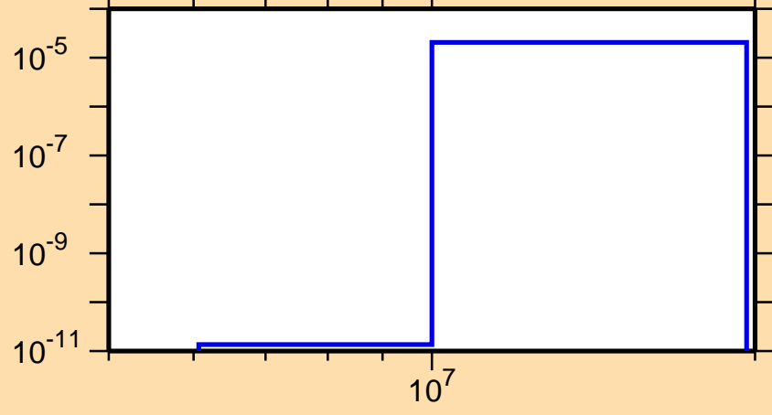
\sigma vs. E for ^{158}\text{Eu}(n,n\alpha)
