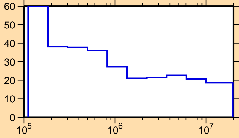
\Delta\sigma/\sigma vs. E for ^{158}\text{Eu}(n,n\text{onel.})
