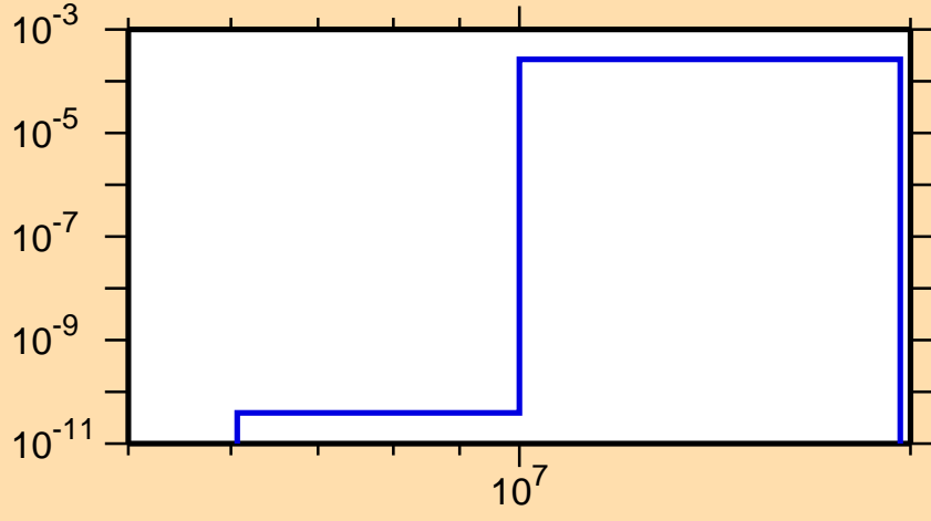
\sigma vs. E for ^{158}\text{Eu}(n,d)
