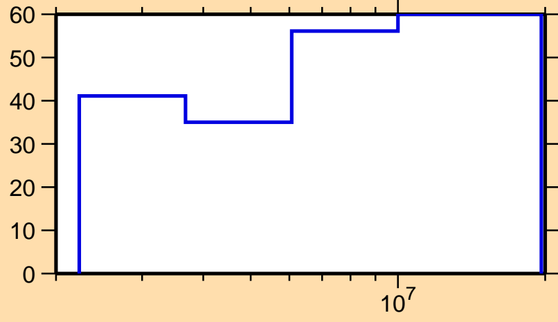
\Delta\sigma/\sigma vs. E for ^{158}\text{Eu}(n,ncont.)
