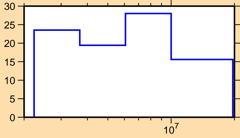
\Delta\sigma/\sigma vs. E for ^{158}\text{Eu}(n,el.)
