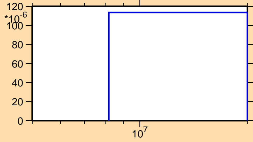
\sigma vs. E for ^{158}\text{Eu}(n,np)
