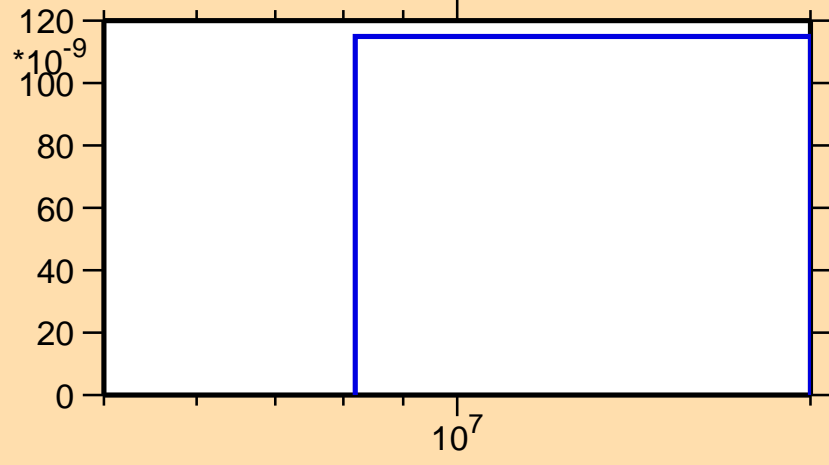
\sigma vs. E for ^{158}\text{Eu}(n,nd)
