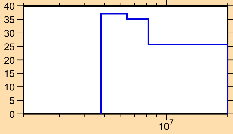
\Delta\sigma/\sigma vs. E for ^{158}\text{Eu}(n,2n)
