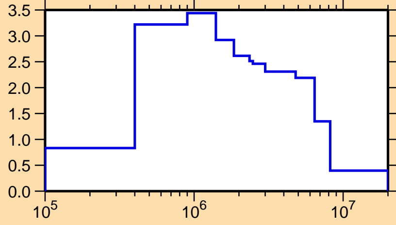
\sigma vs. E for ^{158}\text{Eu}(n,\text{inel.})
