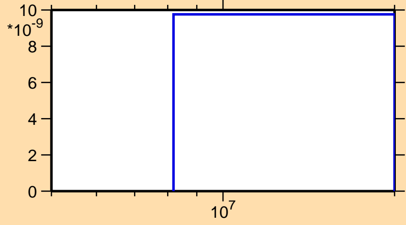
\sigma vs. E for ^{158}\text{Eu}(n,nt)
