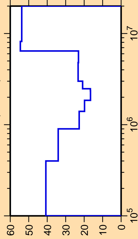
\Delta\sigma/\sigma vs. E for ^{158}\text{Eu}(n,\text{inel.})
