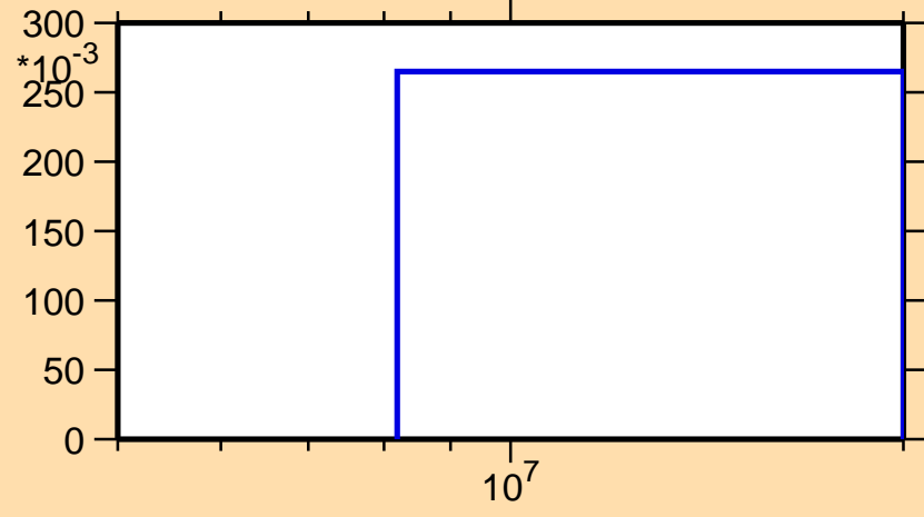
\sigma vs. E for ^{159}\text{Eu}(n,3n)
