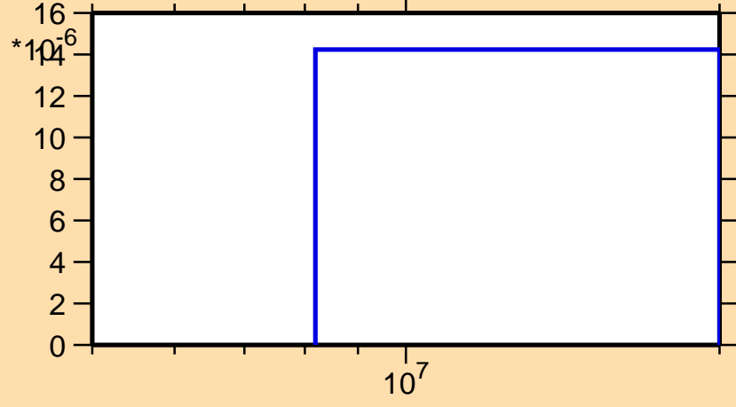
\sigma vs. E for ^{159}\text{Eu}(n,t)
