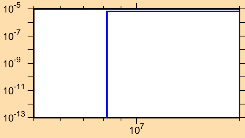
\sigma vs. E for ^{159}\text{Eu}(n,n\alpha)
