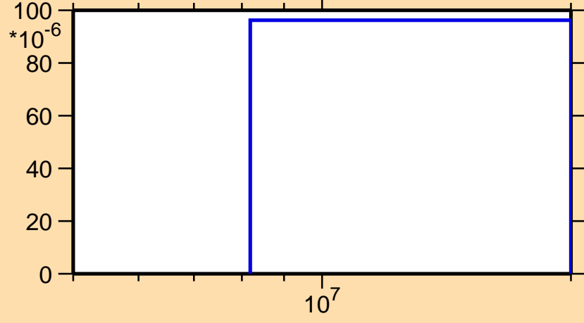
\sigma vs. E for ^{159}\text{Eu}(n,d)
