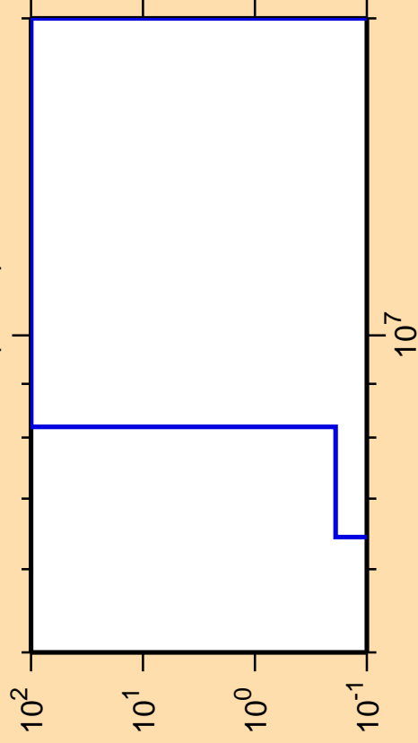
\Delta\sigma/\sigma vs. E for ^{159}\text{Eu}(n,n\alpha)
