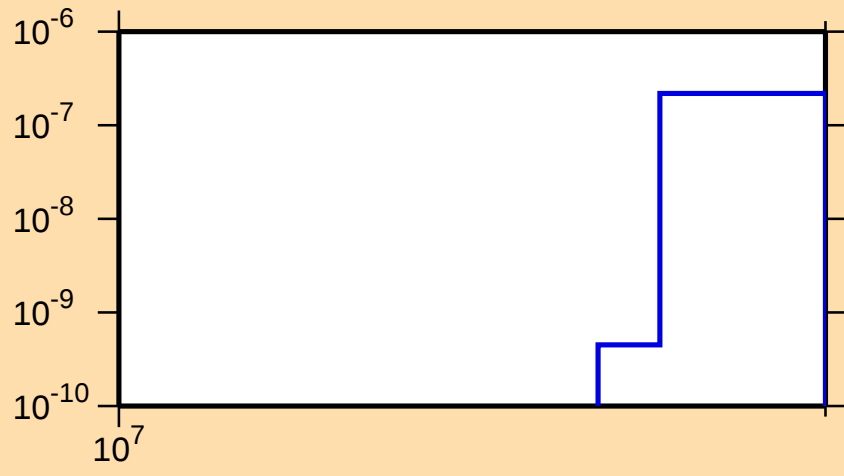
\sigma vs. E for ^{160}\text{Eu}(n,2np)
