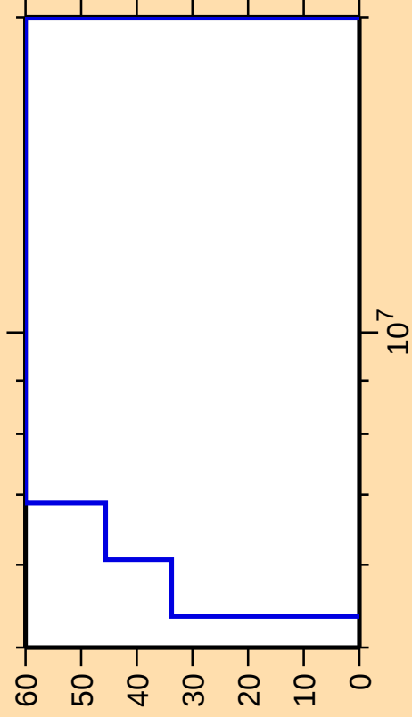
\Delta\sigma/\sigma vs. E for ^{160}\text{Eu}(n,n\text{cont.})
