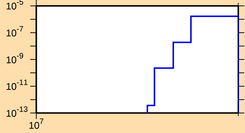
\sigma vs. E for ^{160}\text{Eu}(n,nt)
