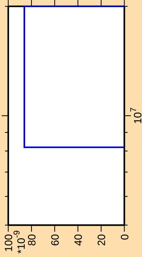
\Delta\sigma/\sigma vs. E for ^{160}\text{Eu} (mt 11)
