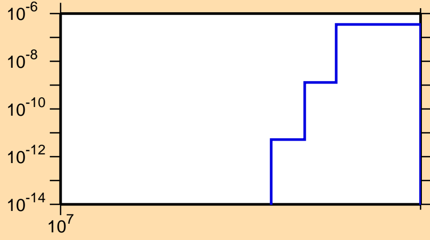
\sigma vs. E for ^{161}\text{Eu}(n,nd)
