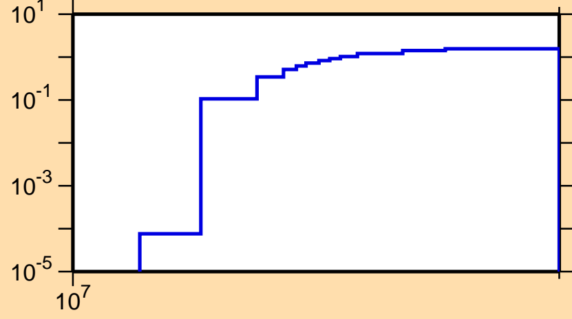
\sigma vs. E for ^{161}\text{Eu}(n,3n)
