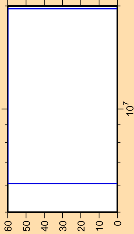
\Delta\sigma/\sigma vs. E for ^{161}\text{Eu}(n,\gamma)
