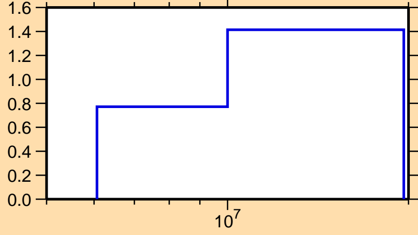
\sigma vs. E for ^{161}\text{Eu}(n,2n)
