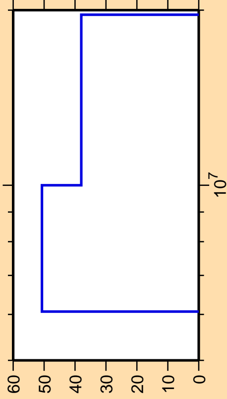
\Delta\sigma/\sigma vs. E for ^{161}\text{Eu}(n,2n)
