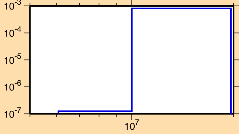
\sigma vs. E for ^{161}\text{Eu}(n,p)
