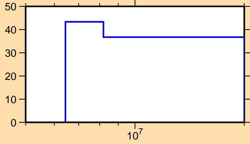
\Delta\sigma/\sigma vs. E for ^{161}\text{Eu}(n,el.)
