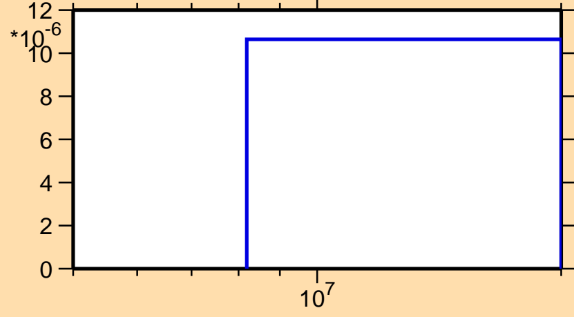
\sigma vs. E for ^{161}\text{Eu}(n,t)
