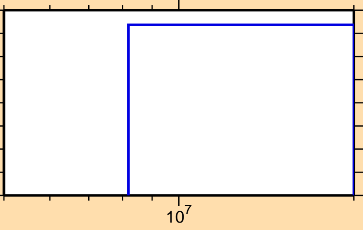
\sigma vs. E for ^{161}\text{Eu}(n,n\alpha)
