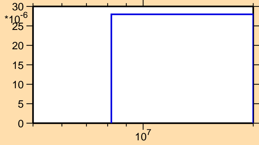
\sigma vs. E for ^{161}\text{Eu}(n,np)
