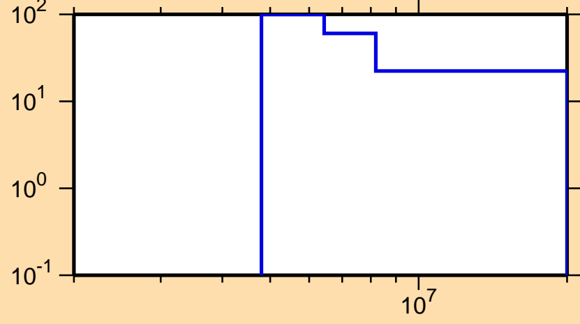
\Delta\sigma/\sigma vs. E for ^{161}\text{Eu}(n,2n)
