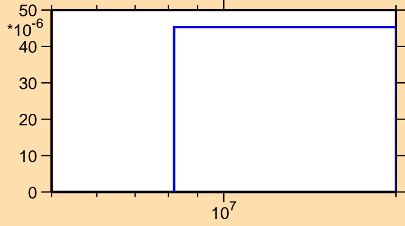
\sigma vs. E for ^{161}\text{Eu}(n,d)
