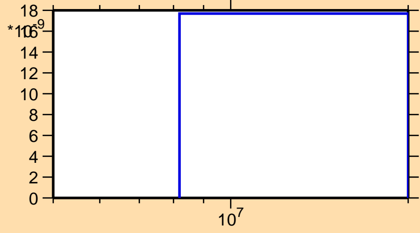
\sigma vs. E for ^{161}\text{Eu}(n,nt)
