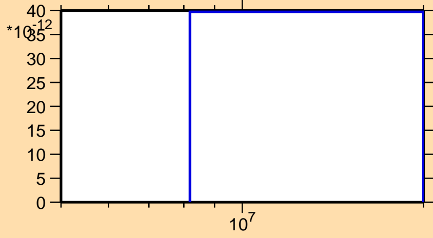
\sigma vs. E for ^{161}\text{Eu}(n,2n\alpha)
