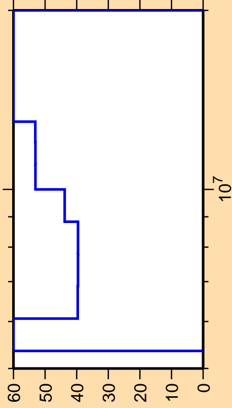
\Delta\sigma/\sigma vs. E for ^{163}\text{Eu}(n,2n)
