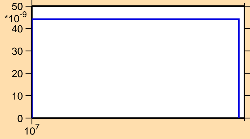
\sigma vs. E for ^{163}\text{Eu}(n,nt)
