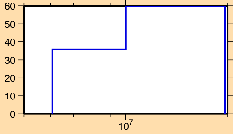
\Delta\sigma/\sigma vs. E for ^{163}\text{Eu}(n,2n)
