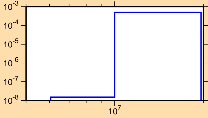
\sigma vs. E for ^{163}\text{Eu}(n,p)
