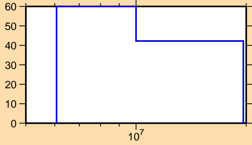
\Delta\sigma/\sigma vs. E for ^{163}\text{Eu}(n,el.)
