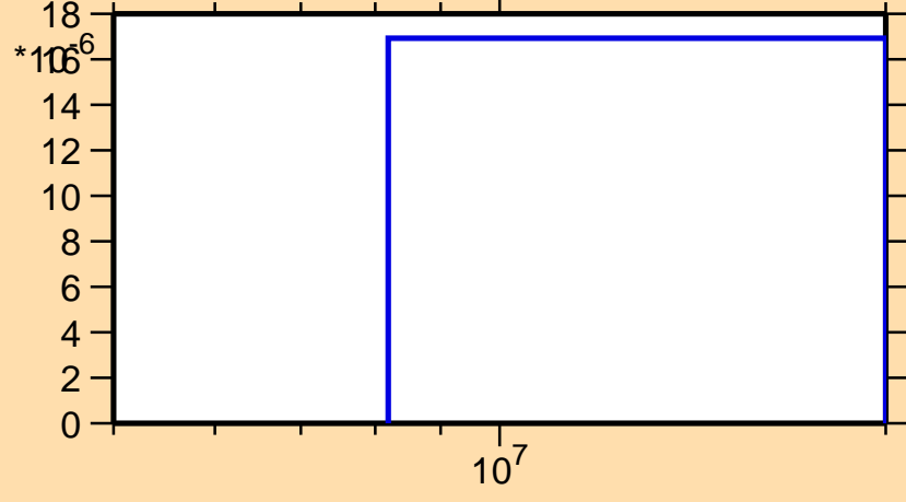
\sigma vs. E for ^{163}\text{Eu}(n,np)
