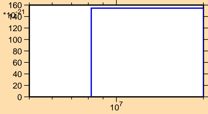
\sigma vs. E for ^{163}\text{Eu} (mt 42)
