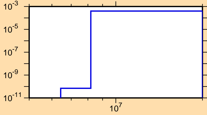
\sigma vs. E for ^{163}\text{Eu}(n,p)
