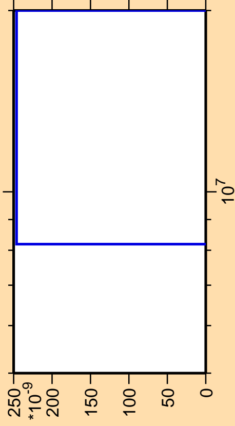
\Delta\sigma/\sigma vs. E for ^{163}\text{Eu} (mt 42)
