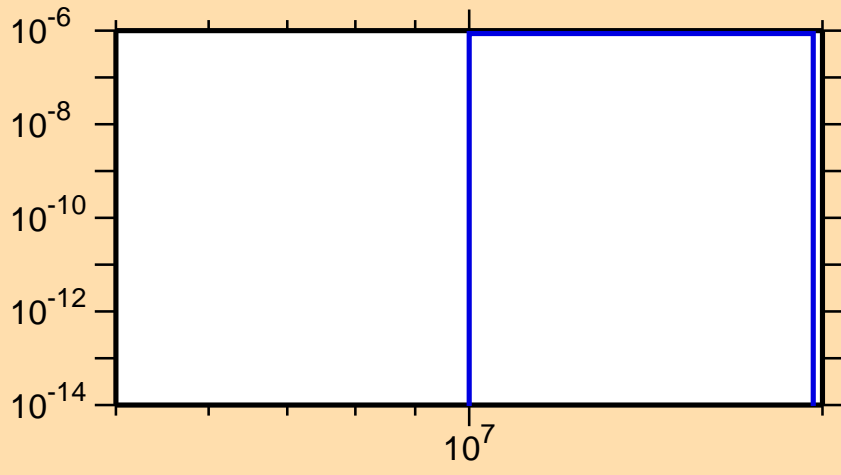
\sigma vs. E for ^{164}\text{Eu}(n,n\alpha)
