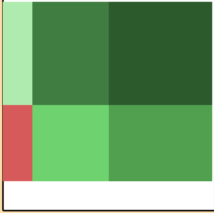
\Delta\sigma/\sigma vs. E for ^{164}\text{Eu}(n,\text{inel.})
