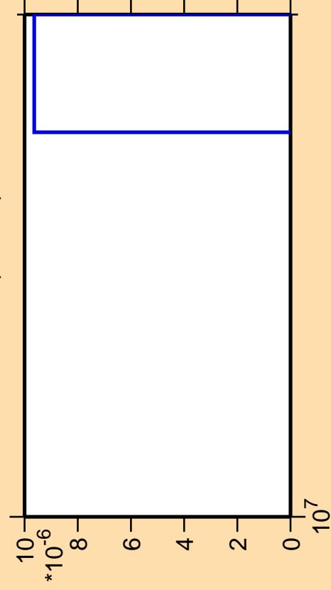
\Delta\sigma/\sigma vs. E for ^{165}\text{Eu} (mt 42)
