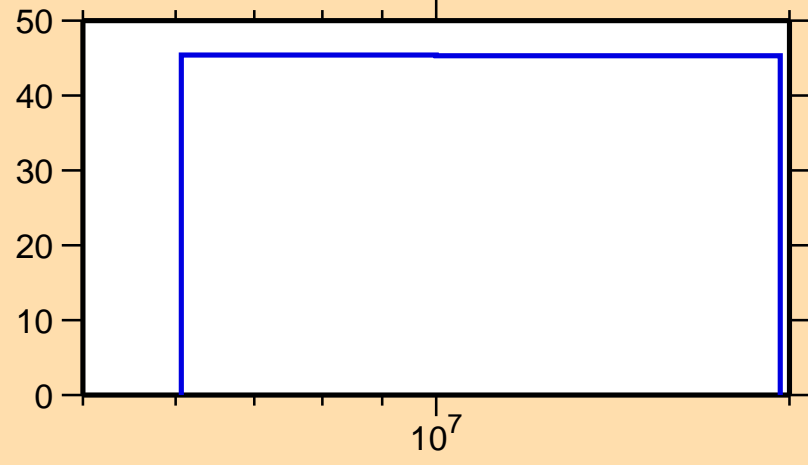
\Delta\sigma/\sigma vs. E for ^{165}\text{Eu}(n,ncont.)
