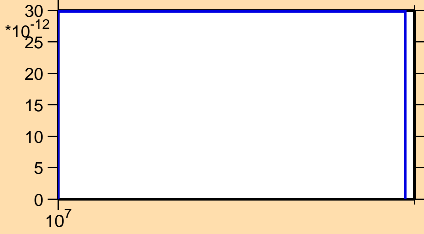
\sigma vs. E for ^{165}\text{Eu}(n,2np)
