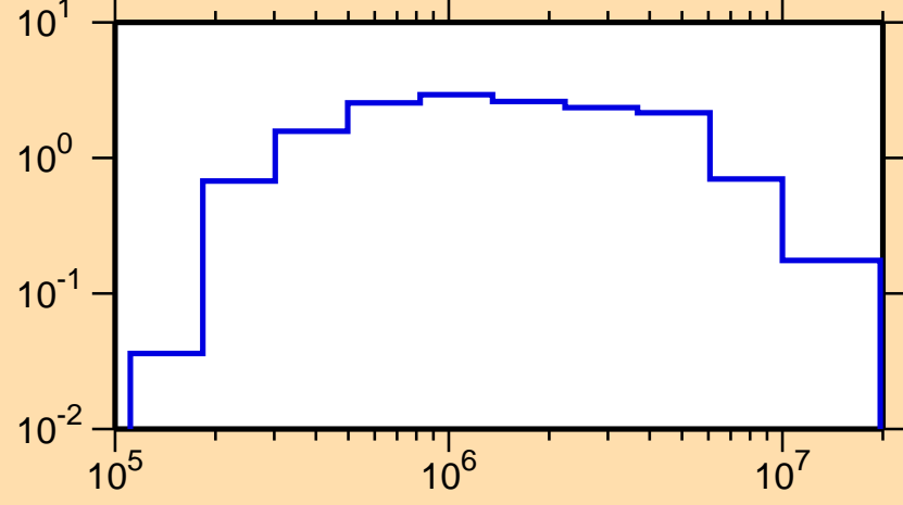
\sigma vs. E for ^{165}\text{Eu}(n,\text{inel.})
