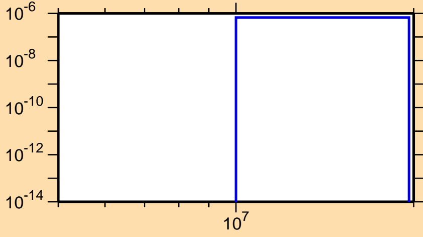
\sigma vs. E for ^{165}\text{Eu}(n,n\alpha)
