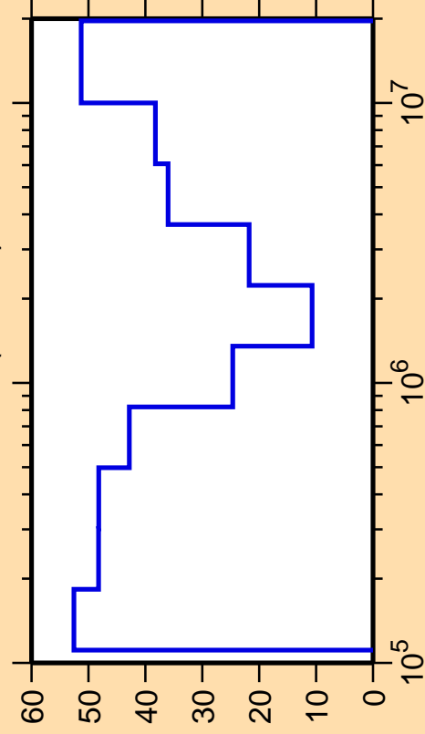
\Delta\sigma/\sigma vs. E for ^{165}\text{Eu}(n,\text{inel.})
