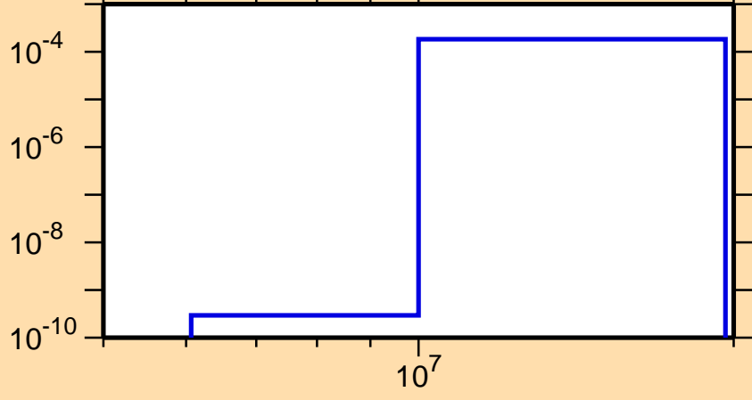
\sigma vs. E for ^{165}\text{Eu}(n,p)
