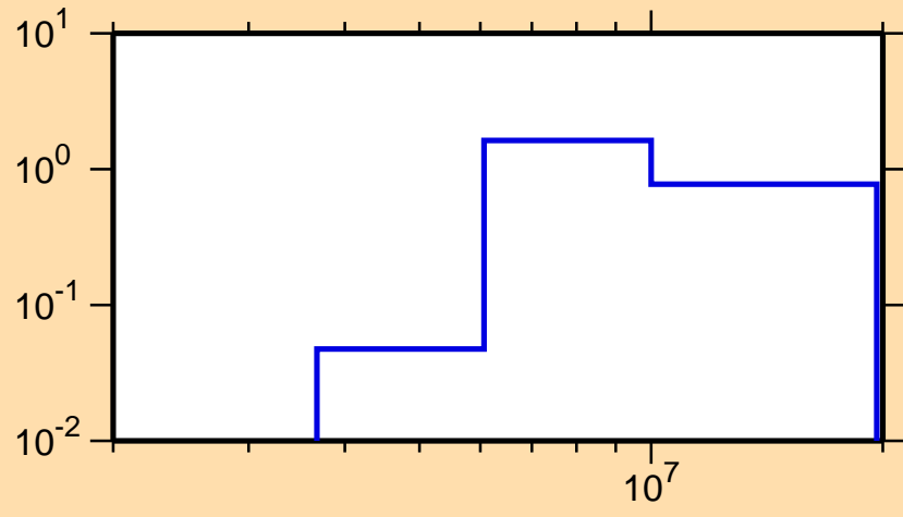
\sigma vs. E for ^{165}\text{Eu}(n,2n)
