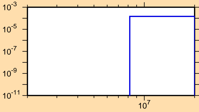
\sigma vs. E for ^{165}\text{Eu}(n,p)
