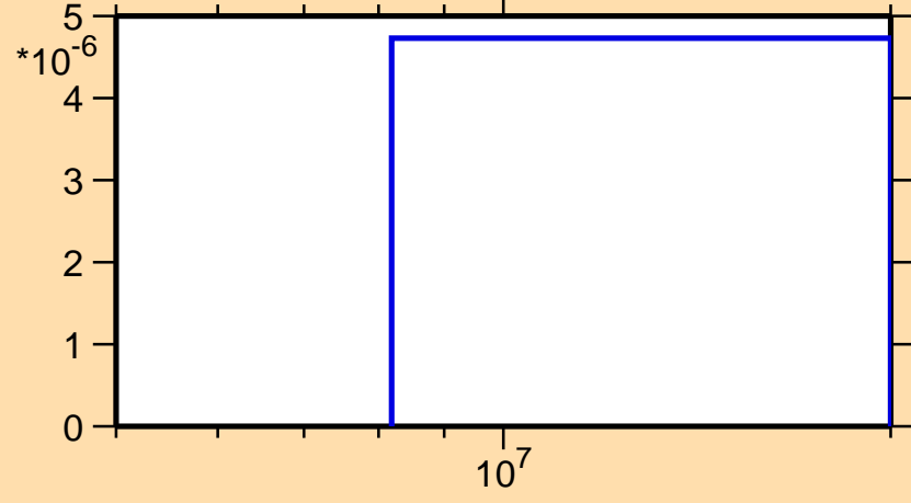
\sigma vs. E for ^{165}\text{Eu}(n,t)
