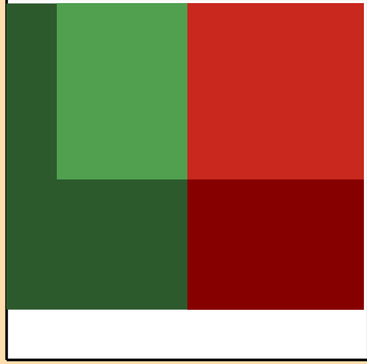
\Delta\sigma/\sigma vs. E for ^{166}\text{Eu}(n,p)
