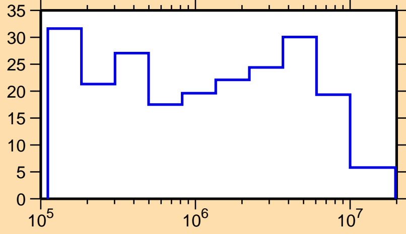
\Delta\sigma/\sigma vs. E for ^{166}\text{Eu}(n, el.)
