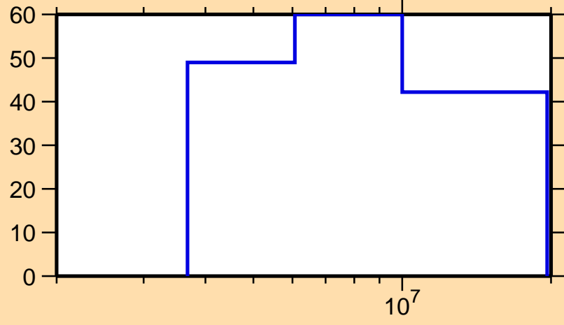
\Delta\sigma/\sigma vs. E for ^{166}\text{Eu}(n,ncont.)
