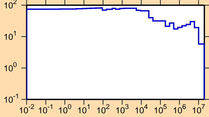
\Delta\sigma/\sigma vs. E for ^{166}\text{Eu}(n,\text{el.})
