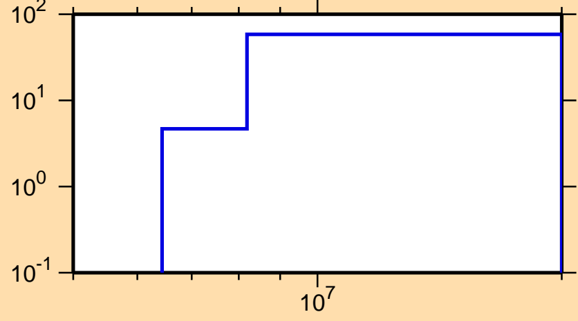
\Delta\sigma/\sigma vs. E for ^{166}\text{Eu}(n,p)
