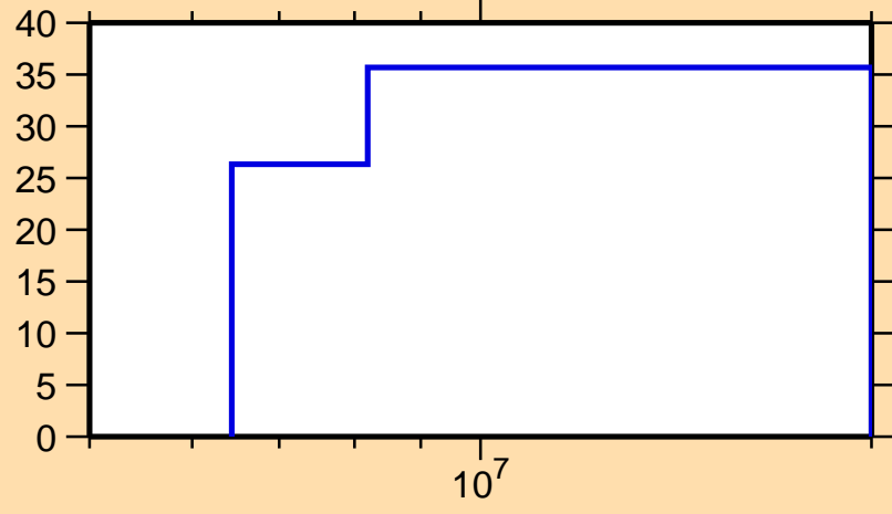
\Delta\sigma/\sigma vs. E for ^{166}\text{Eu}(n,2n)
