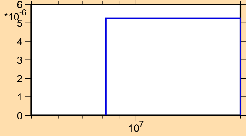
\sigma vs. E for ^{166}\text{Eu}(n,d)
