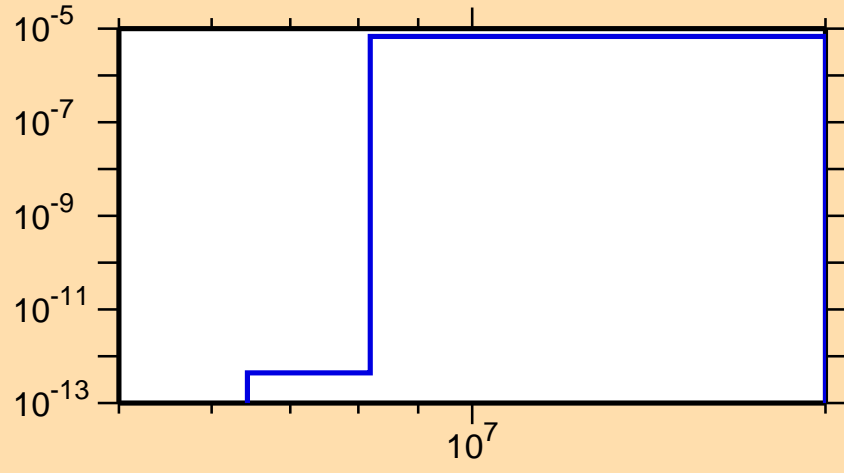
\sigma vs. E for ^{166}\text{Eu}(n,\alpha)
