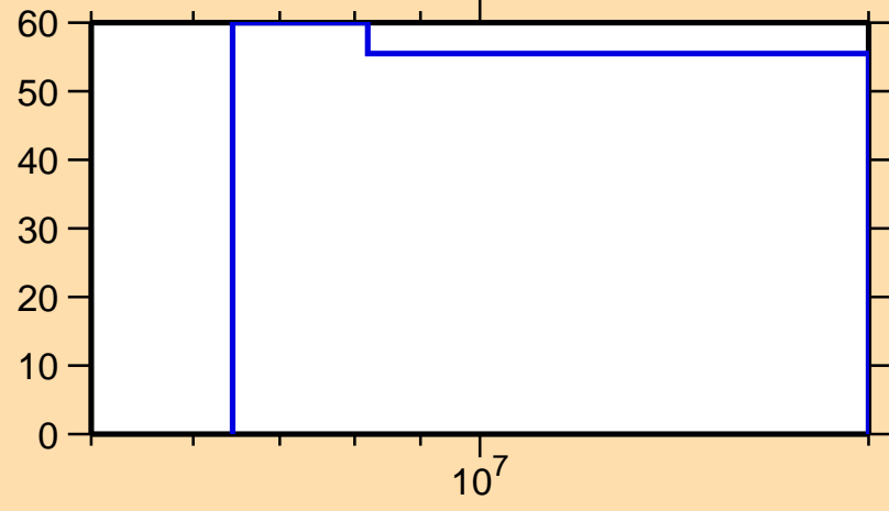
\Delta\sigma/\sigma vs. E for ^{166}\text{Eu}(n,n\text{cont.})
