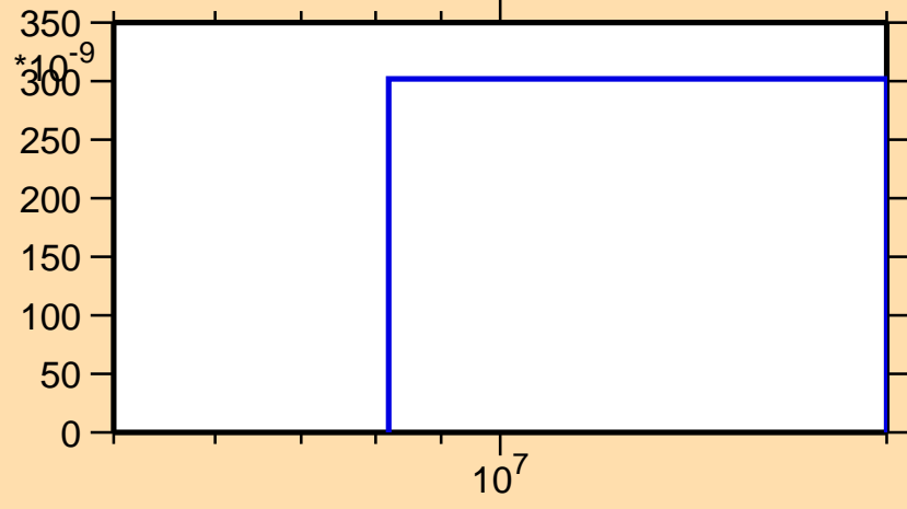
\sigma vs. E for ^{166}\text{Eu}(n,n\alpha)
