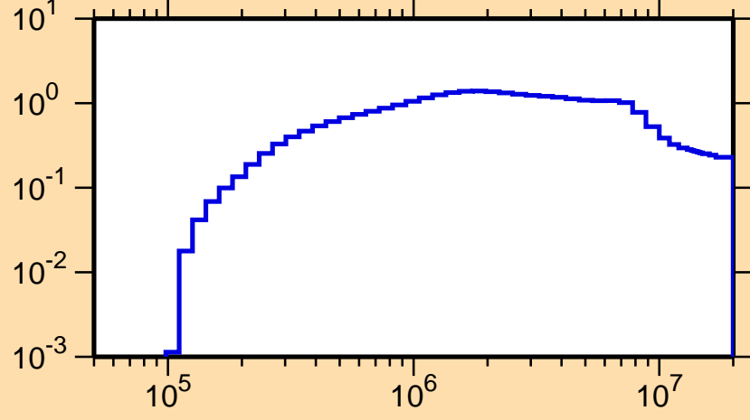
\sigma vs. E for ^{245}\text{Fm}(n,\text{inel.})
