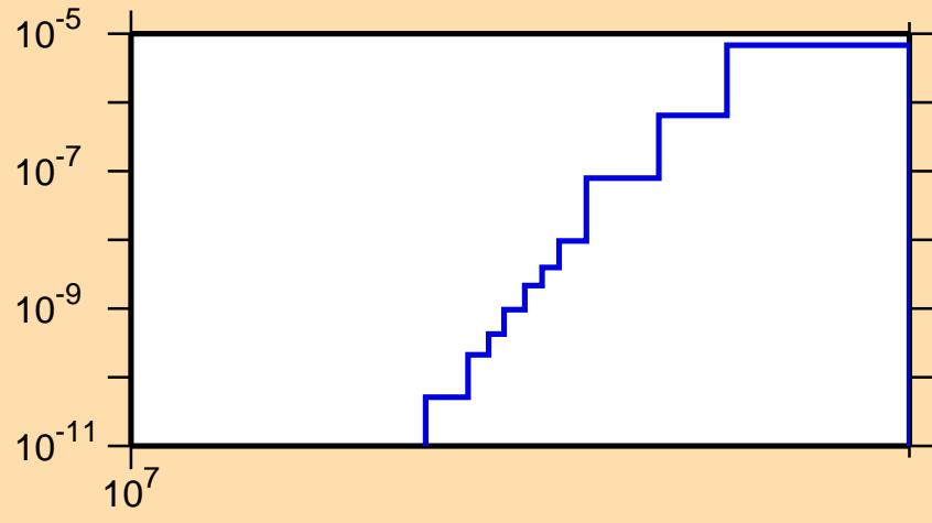
\sigma vs. E for ^{245}\text{Fm}(n,nd)
