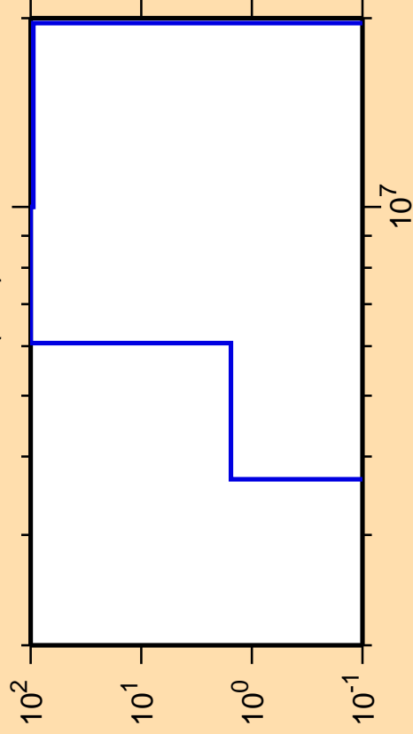
\Delta\sigma/\sigma vs. E for ^{245}\text{Fm}(n,d)
