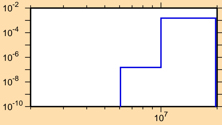
\sigma vs. E for ^{245}\text{Fm}(n,d)
