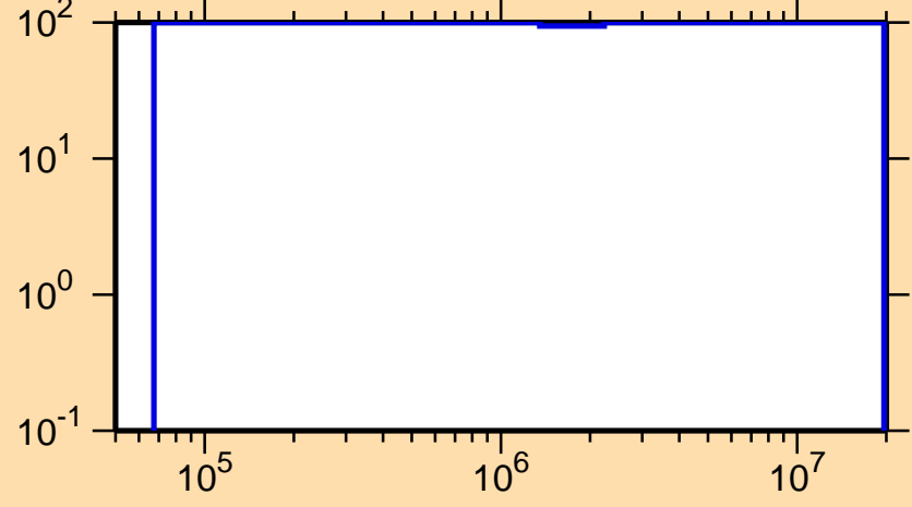
\Delta\sigma/\sigma vs. E for ^{245}\text{Fm}(n,\text{inel.})
