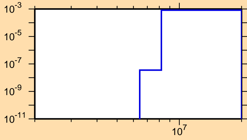
\sigma vs. E for ^{245}\text{Fm}(n,np)
