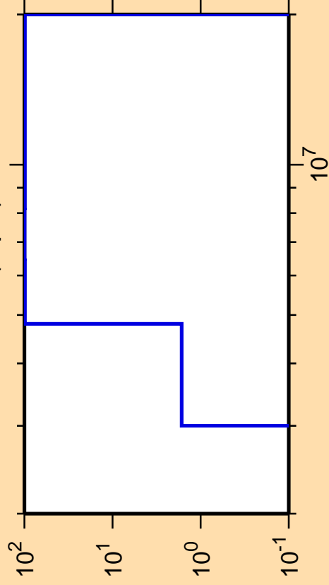
\Delta\sigma/\sigma vs. E for ^{245}\text{Fm}(n,p\alpha)
