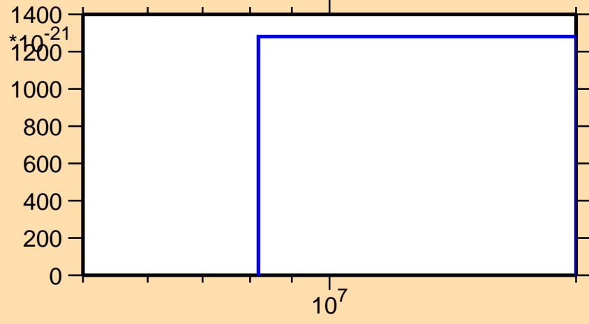
\sigma vs. E for ^{245}\text{Fm} (mt 42)
