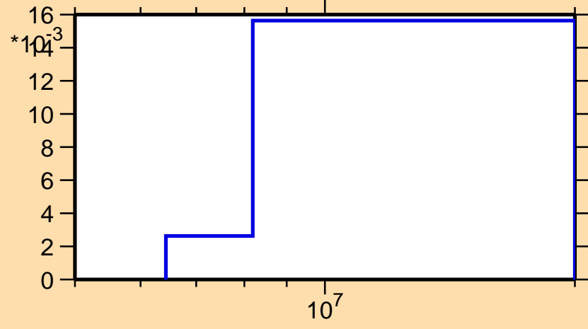
\sigma vs. E for ^{245}\text{Fm}(n,2n\alpha)
