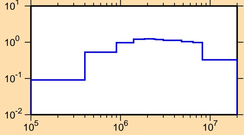
\sigma vs. E for ^{245}\text{Fm}(n,n\text{cont.})
