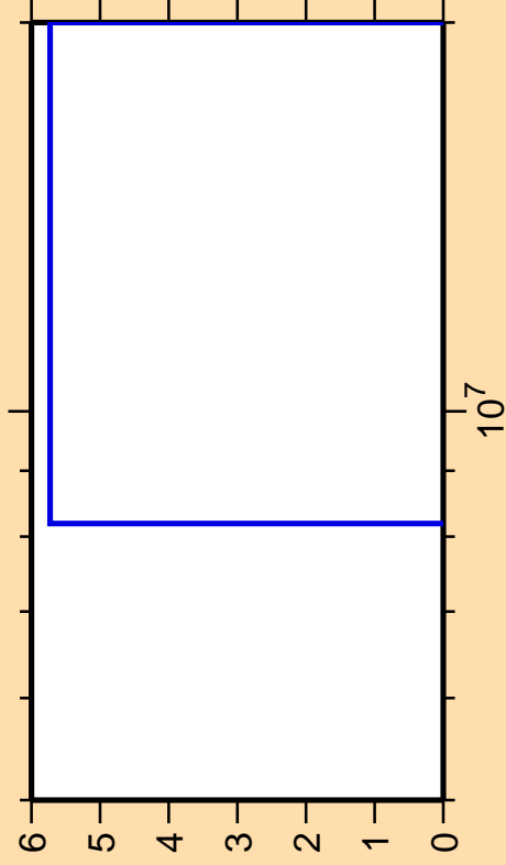
\Delta\sigma/\sigma vs. E for ^{245}\text{Fm} (mt 34)
