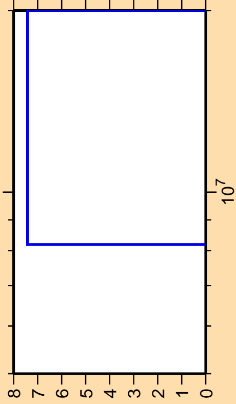
\Delta\sigma/\sigma vs. E for ^{245}\text{Fm} (mt 45)
