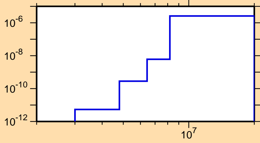
\sigma vs. E for ^{245}\text{Fm}(n,p\alpha)
