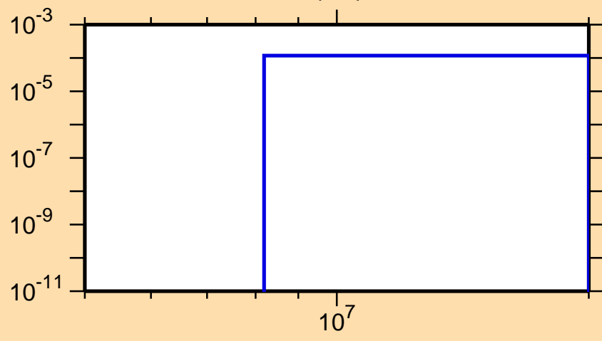
\sigma vs. E for ^{245}\text{Fm}(n,t)
