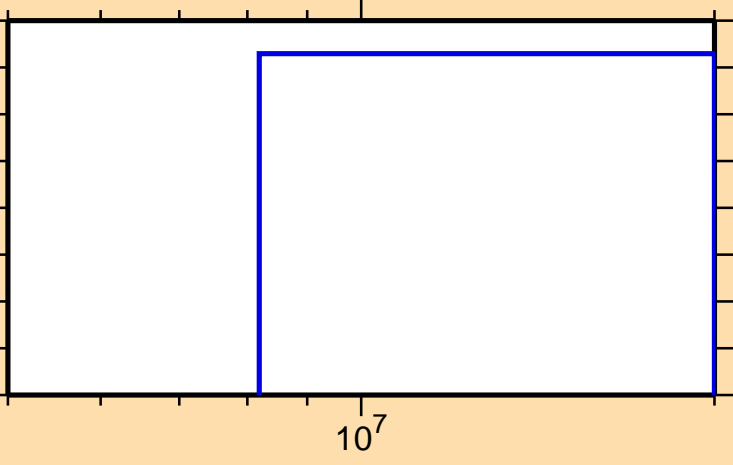
\sigma vs. E for ^{245}\text{Fm}(n,3n)
