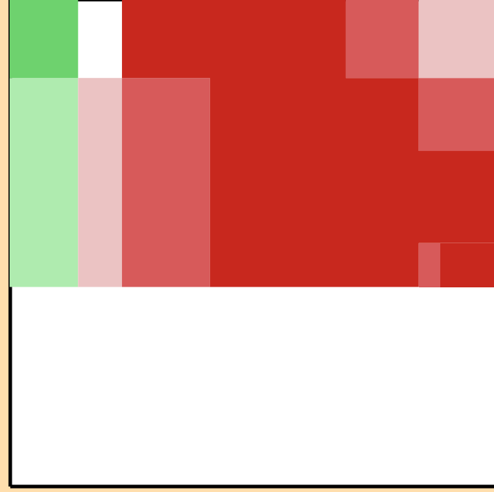
\Delta\sigma/\sigma vs. E for ^{246}\text{Fm}(n,\text{el.})
