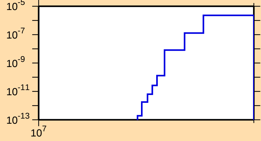
\sigma vs. E for ^{246}\text{Fm}(n,2np)
