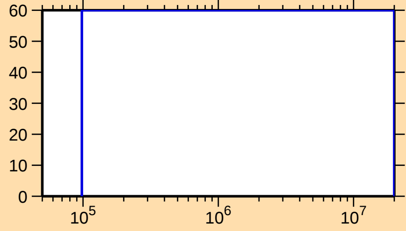
\Delta\sigma/\sigma vs. E for ^{246}\text{Fm}(n,n_1)
