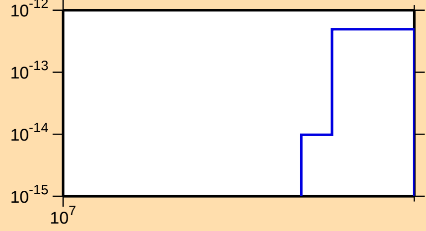
\sigma vs. E for ^{246}\text{Fm}(n,\text{pt})
