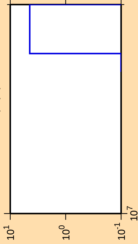
\Delta\sigma/\sigma vs. E for ^{246}\text{Fm}(n,\text{pt})
