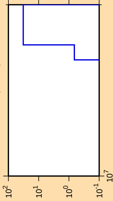
\Delta\sigma/\sigma vs. E for ^{246}\text{Fm}(\text{mt } 34)
