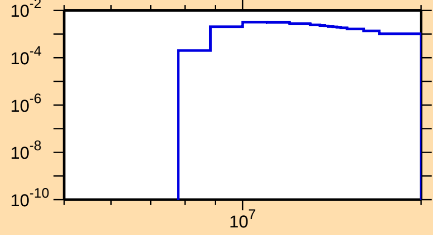
\sigma vs. E for ^{246}\text{Fm}(n,2n\alpha)
