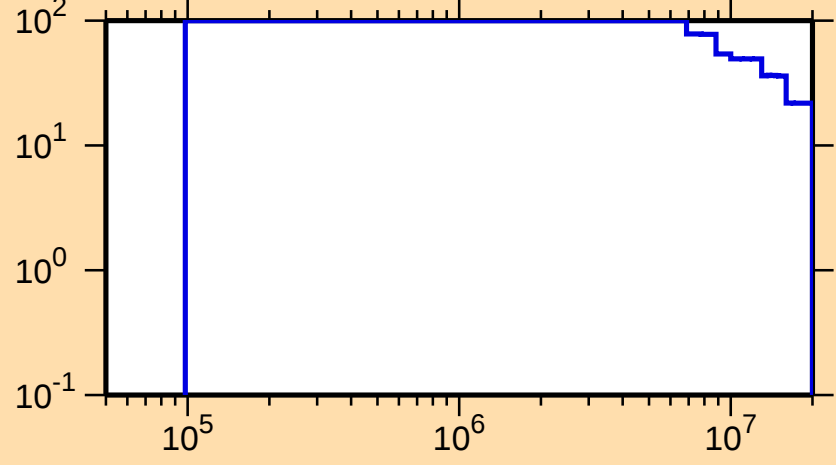
\Delta\sigma/\sigma vs. E for ^{246}\text{Fm}(n,f)
