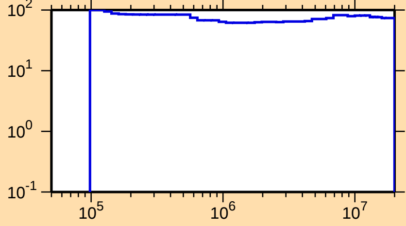
\Delta\sigma/\sigma vs. E for ^{246}\text{Fm}(n,\text{inel.})
