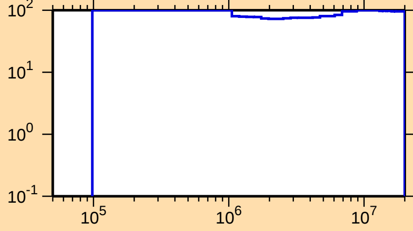
\Delta\sigma/\sigma vs. E for ^{246}\text{Fm}(n,n\text{cont.})
