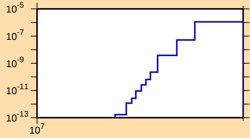
\sigma vs. E for ^{246}\text{Fm}(n,nd)
