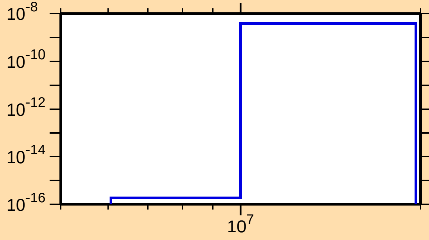
\sigma vs. E for ^{246}\text{Fm}(\text{mt } 45)
