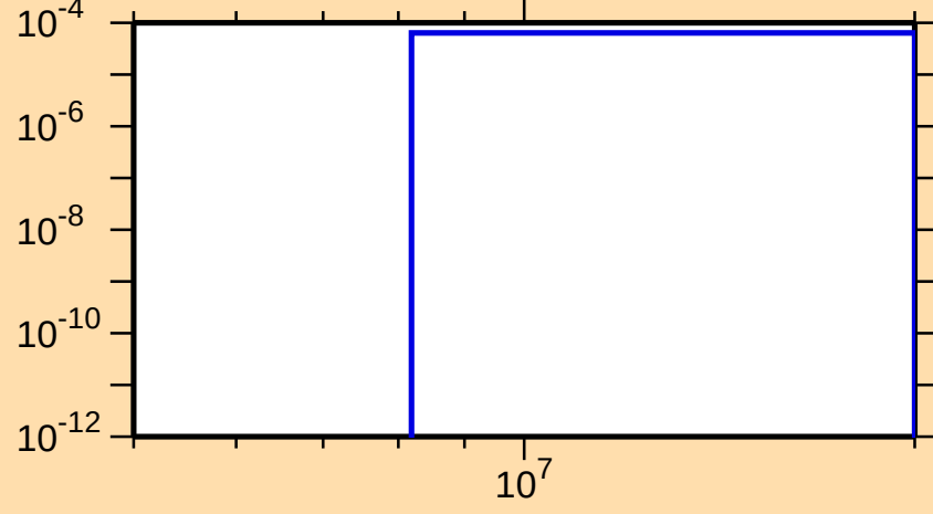
\sigma vs. E for ^{246}\text{Fm}(n,t)
