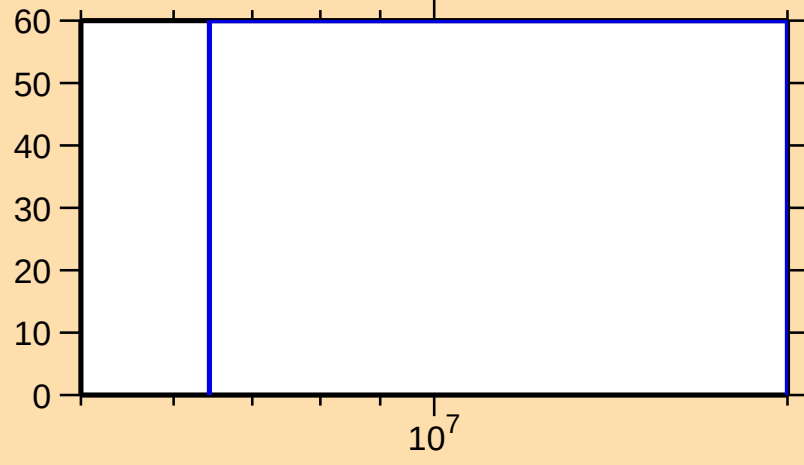
\Delta\sigma/\sigma vs. E for ^{246}\text{Fm}(n,2n)
