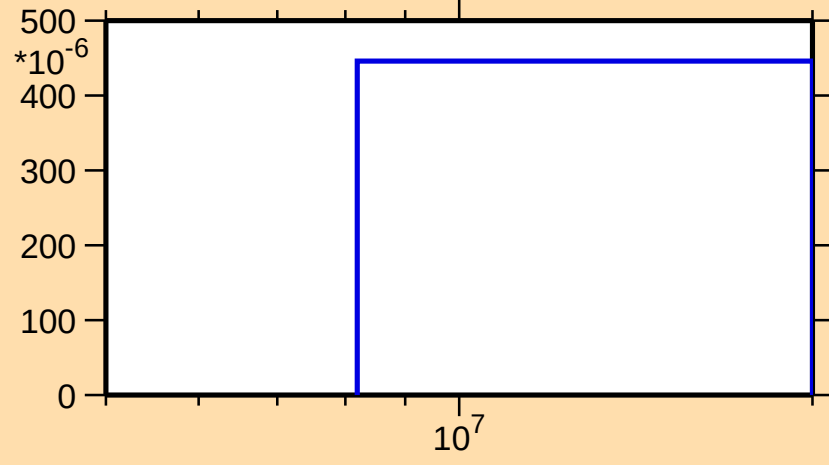
\sigma vs. E for ^{246}\text{Fm}(n,3n\alpha)
