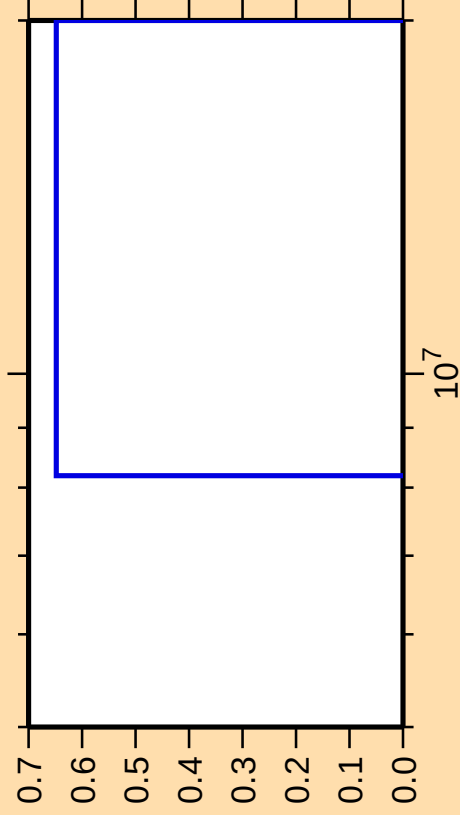
\Delta\sigma/\sigma vs. E for ^{246}\text{Fm}(n,\text{pd})
