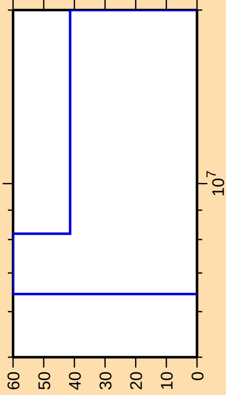
\Delta\sigma/\sigma vs. E for ^{246}\text{Fm}(n,f)
