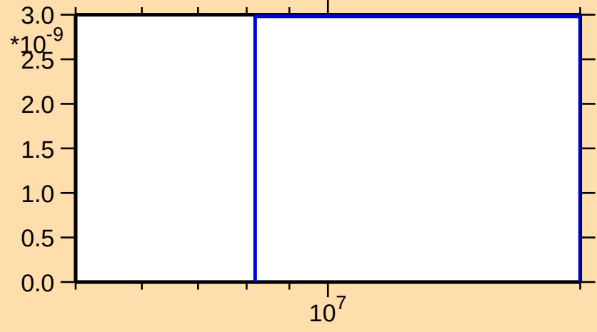
\sigma vs. E for ^{246}\text{Fm}(\text{mt117})
