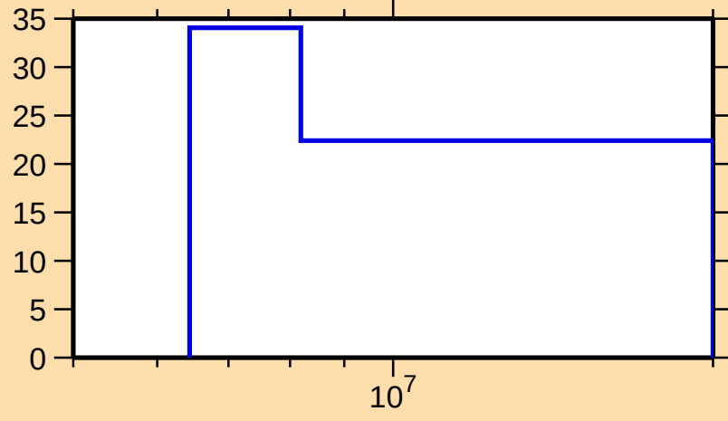
\Delta\sigma/\sigma vs. E for ^{246}\text{Fm}(n,\text{el.})
