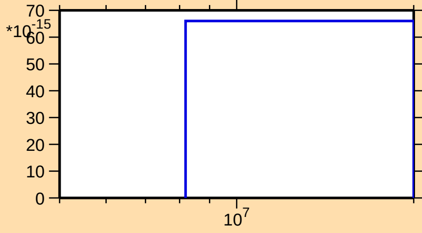
\sigma vs. E for ^{246}\text{Fm}(\text{mt } 34)
