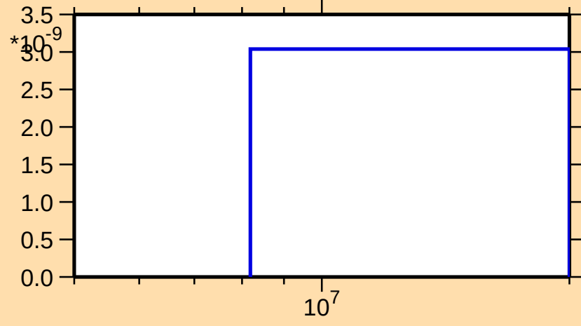
\sigma vs. E for ^{246}\text{Fm}(\text{mt } 45)
