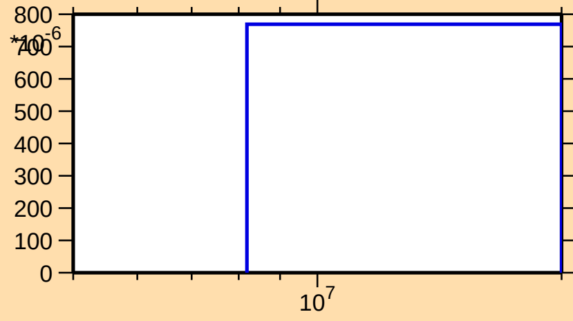
\sigma vs. E for ^{246}\text{Fm}(n,3n)
