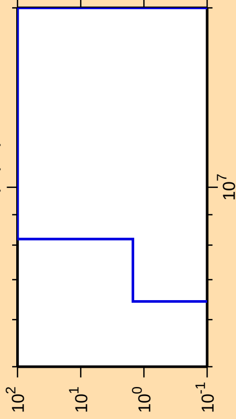
\Delta\sigma/\sigma vs. E for ^{246}\text{Fm}(n,p\alpha)
