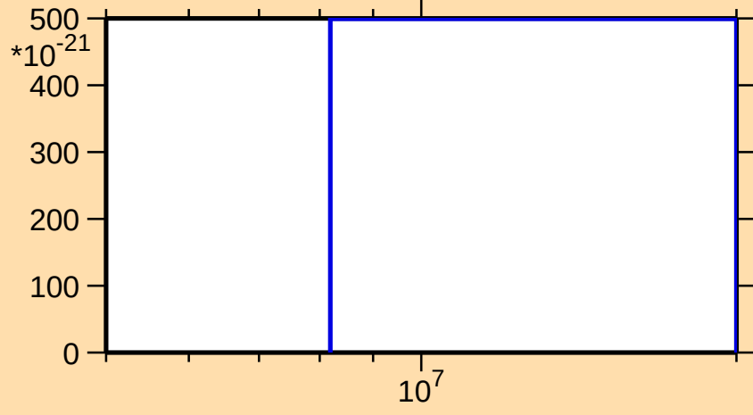
\sigma vs. E for ^{246}\text{Fm}(\text{mt } 42)
