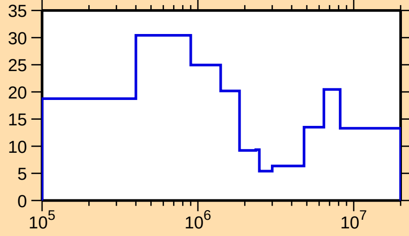
\Delta\sigma/\sigma vs. E for ^{246}\text{Fm}(n,\text{tot.})
