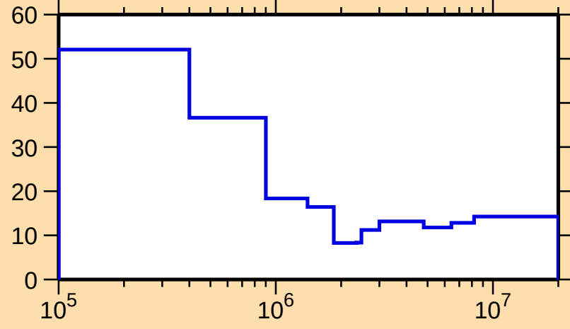
\Delta\sigma/\sigma vs. E for ^{246}\text{Fm}(n,\text{nonel.})
