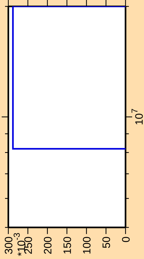
\Delta\sigma/\sigma vs. E for ^{246}\text{Fm}(\text{mt } 34)
