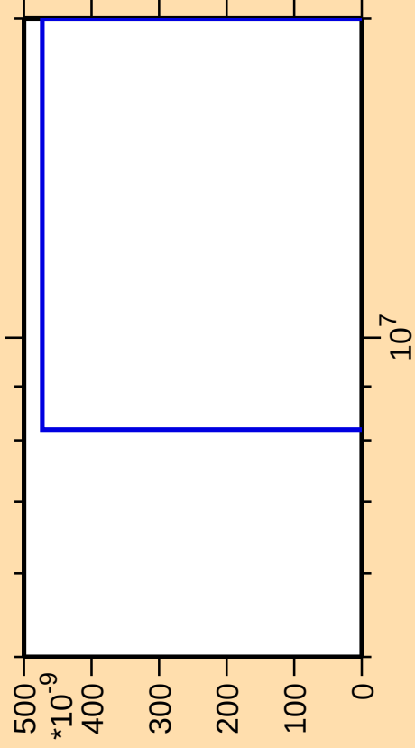
\Delta\sigma/\sigma vs. E for ^{246}\text{Fm}(\text{mt } 42)
