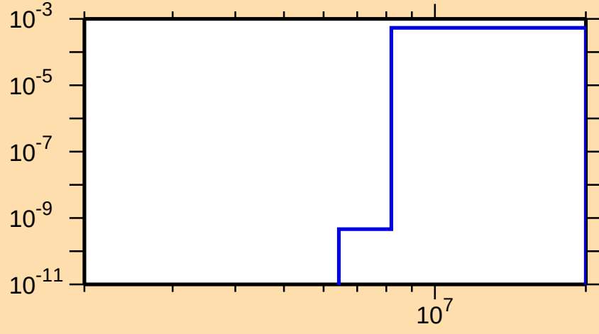
\sigma vs. E for ^{246}\text{Fm}(n,d)
