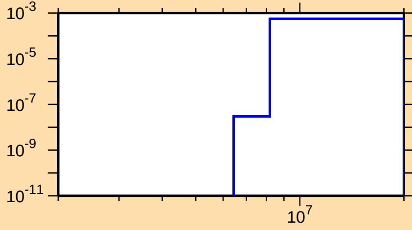
\sigma vs. E for ^{246}\text{Fm}(n,np)
