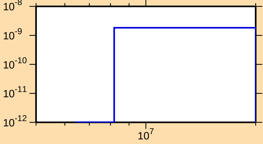
\sigma vs. E for ^{246}\text{Fm}(n,p\alpha)
