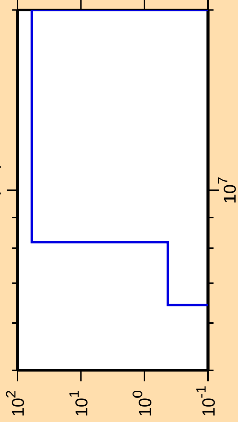
\Delta\sigma/\sigma vs. E for ^{246}\text{Fm}(n,t)
