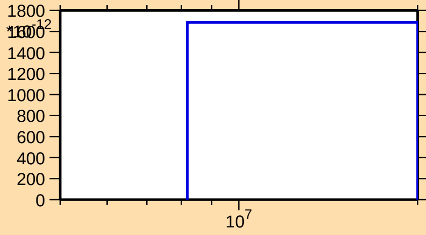
\sigma vs. E for ^{246}\text{Fm}(n,\text{He}3)
