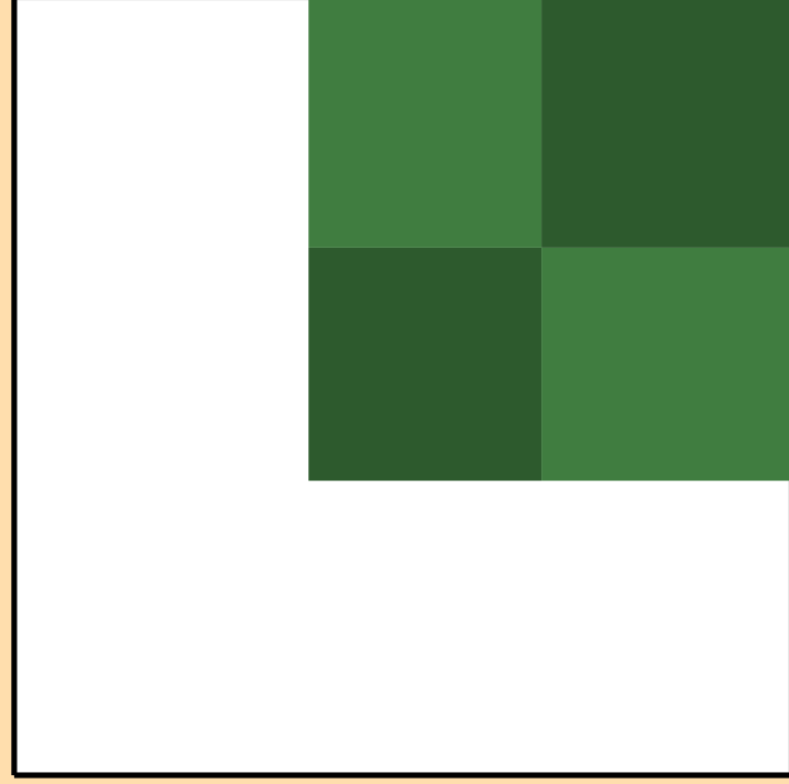
\sigma vs. E for ^{247}\text{Fm}(n,3n\alpha)
