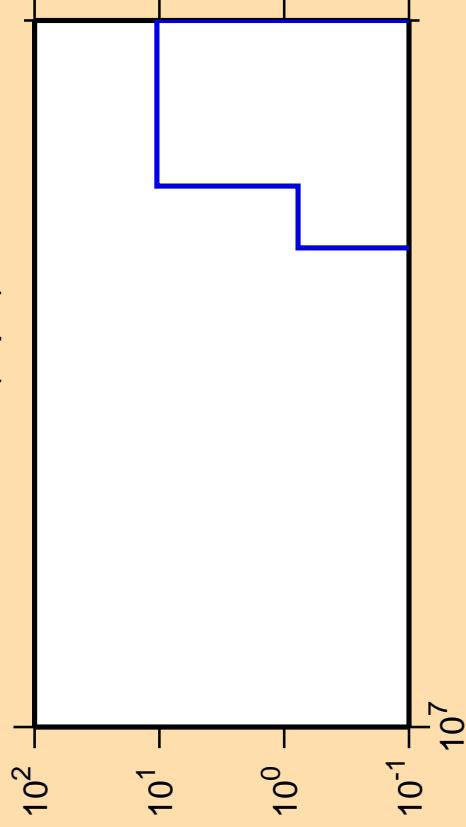
\Delta\sigma/\sigma vs. E for ^{247}\text{Fm}(n,pd)
