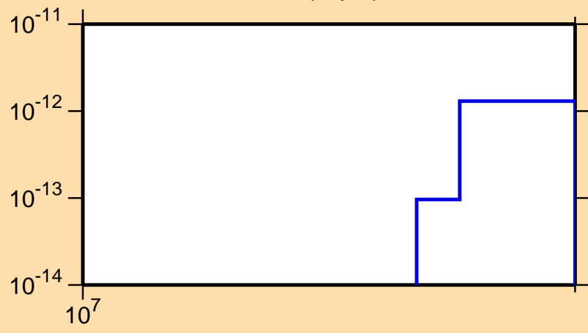
\sigma vs. E for ^{247}\text{Fm}(n,pd)
