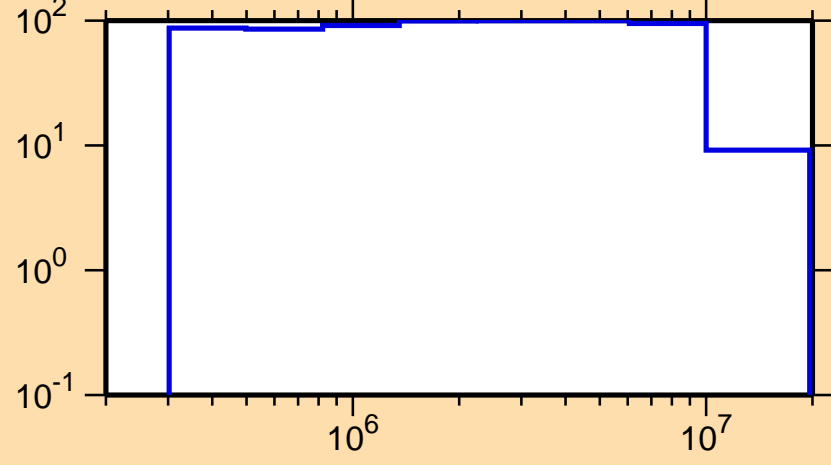
\Delta\sigma/\sigma vs. E for ^{247}\text{Fm}(n,n_1)
