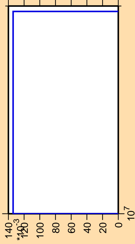
\Delta\sigma/\sigma vs. E for ^{247}\text{Fm}(n,pd)
