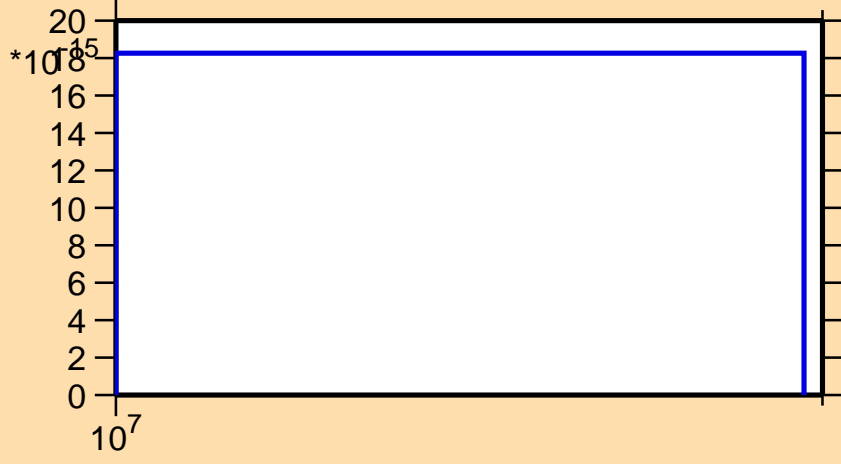
\sigma vs. E for ^{247}\text{Fm}(n,pd)
