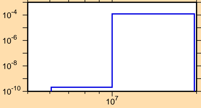
\sigma vs. E for ^{247}\text{Fm}(n,t)
