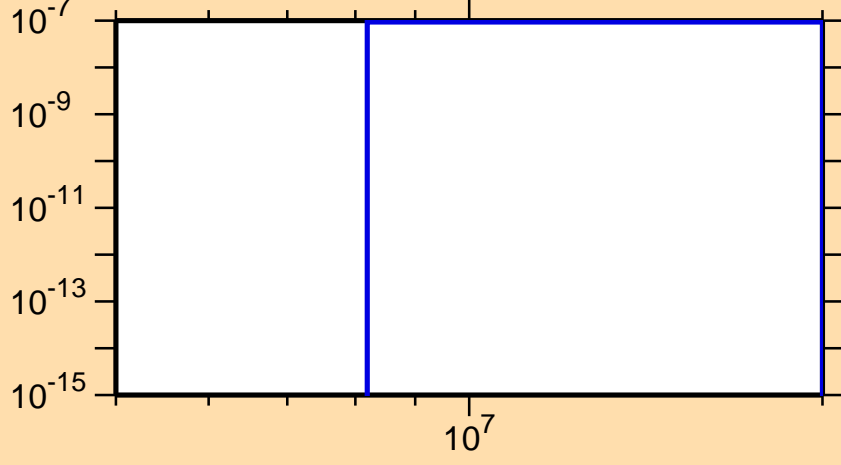
\sigma vs. E for ^{247}\text{Fm}(n,\text{nd})
