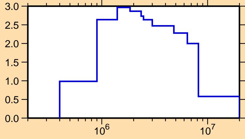
\sigma vs. E for ^{247}\text{Fm}(n,\text{inel.})
