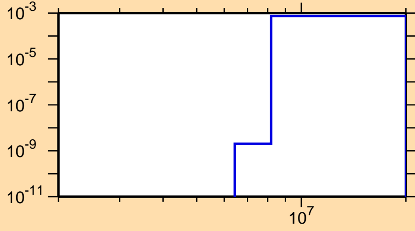
\sigma vs. E for ^{247}\text{Fm}(n,d)
