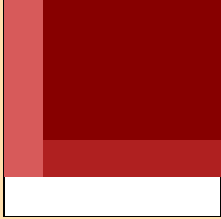
\Delta\sigma/\sigma vs. E for ^{247}\text{Fm}(n,\text{el.})
