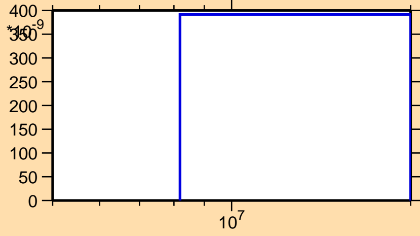
\sigma vs. E for ^{247}\text{Fm}(n,\text{nd})
