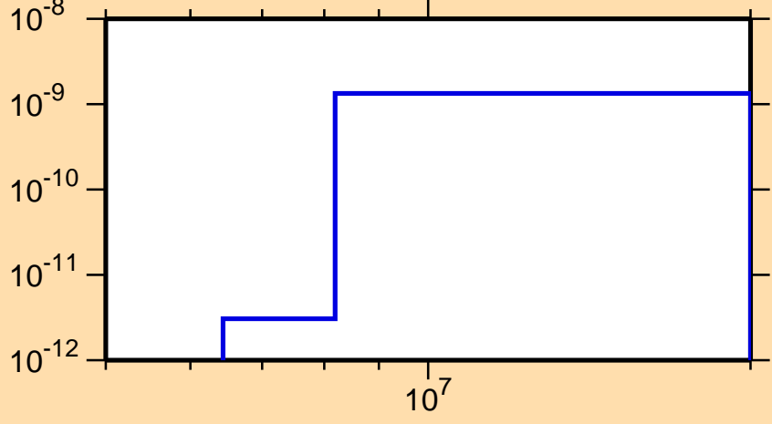
\sigma vs. E for ^{247}\text{Fm}(n,p\alpha)
