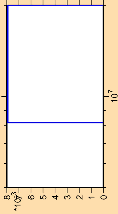
\Delta\sigma/\sigma vs. E for ^{247}\text{Fm}(\text{mt } 11)
