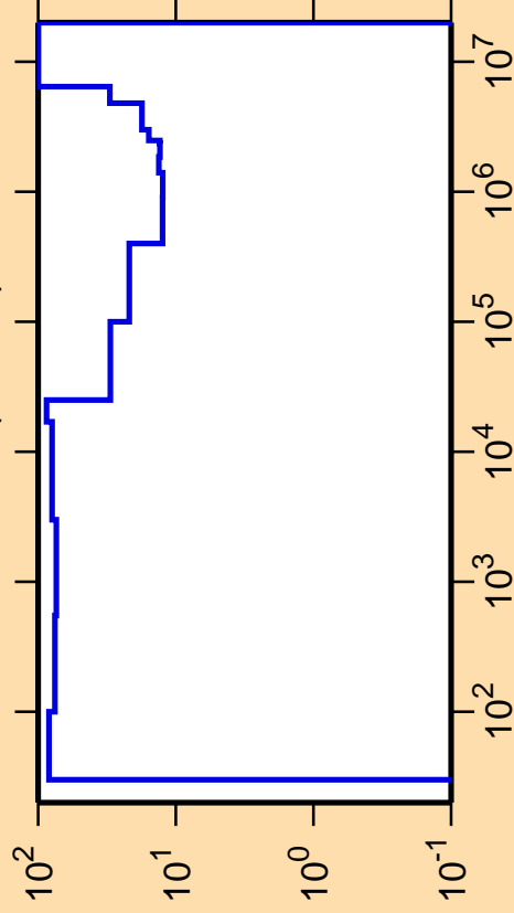
\Delta\sigma/\sigma vs. E for ^{247}\text{Fm}(n,\text{inel.})
