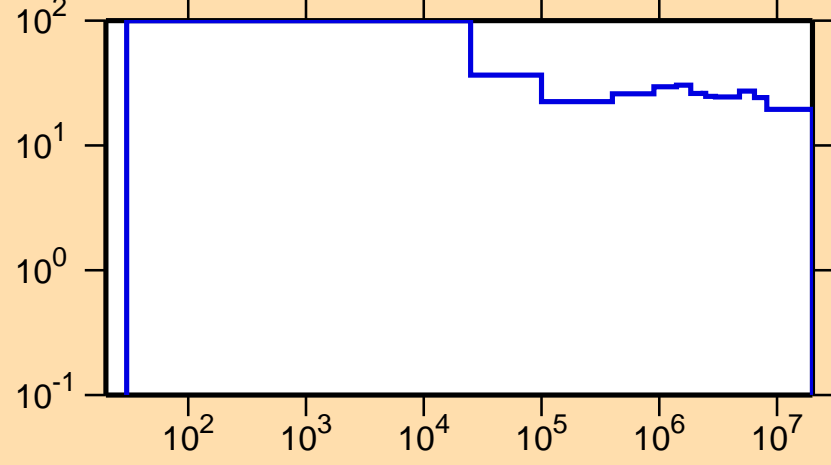
\Delta\sigma/\sigma vs. E for ^{247}\text{Fm}(n,\text{nonel.})
