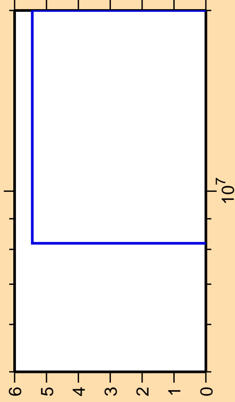
\Delta\sigma/\sigma vs. E for ^{247}\text{Fm}(n,pt)
