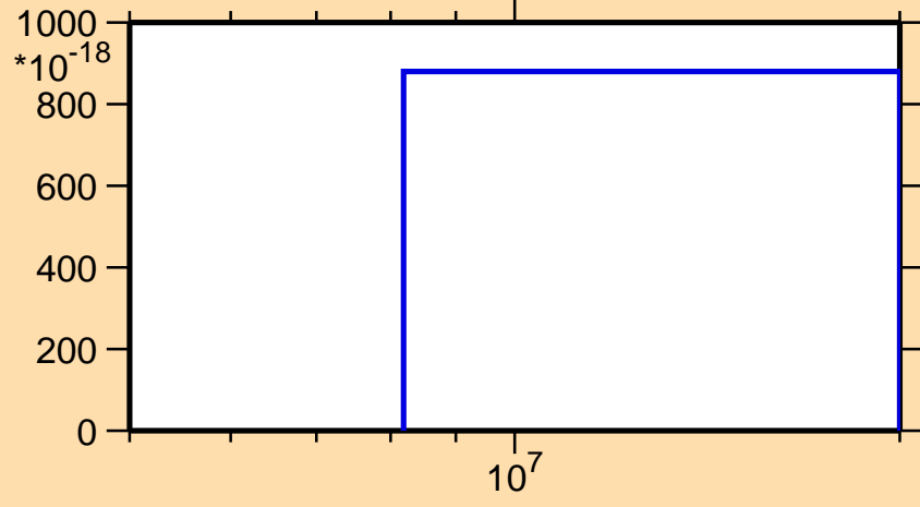
\sigma vs. E for ^{247}\text{Fm}(\text{mt } 11)
