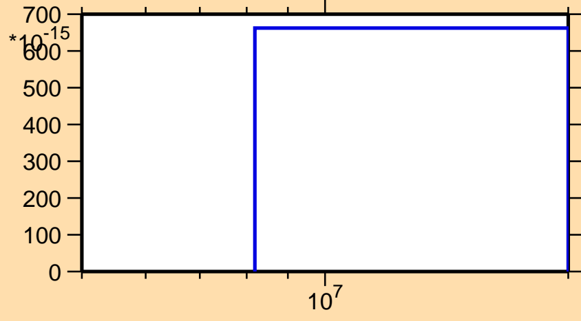
\sigma vs. E for ^{247}\text{Fm}(n,pt)
