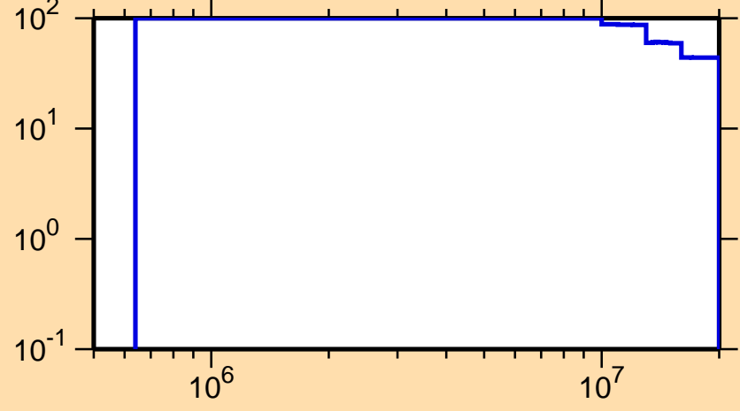
\Delta\sigma/\sigma vs. E for ^{248}\text{Fm}(n,f)
