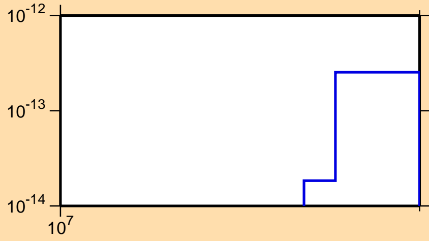
\sigma vs. E for ^{248}\text{Fm}(n,pd)
