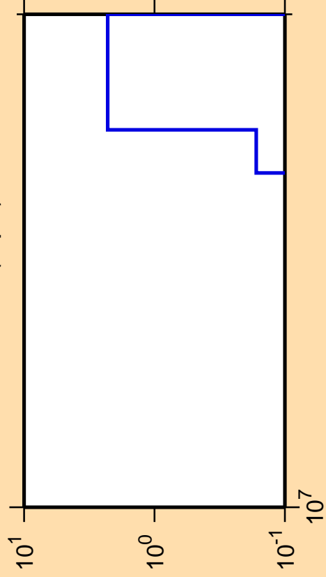
\Delta\sigma/\sigma vs. E for ^{248}\text{Fm}(n,pd)
