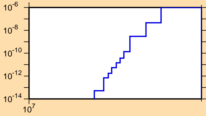
\sigma vs. E for ^{248}\text{Fm}(n,nd)
