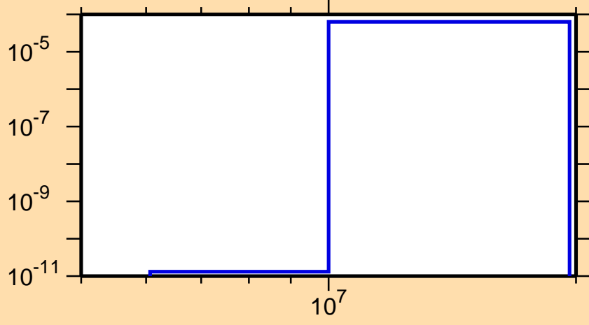
\sigma vs. E for ^{248}\text{Fm}(n,t)
