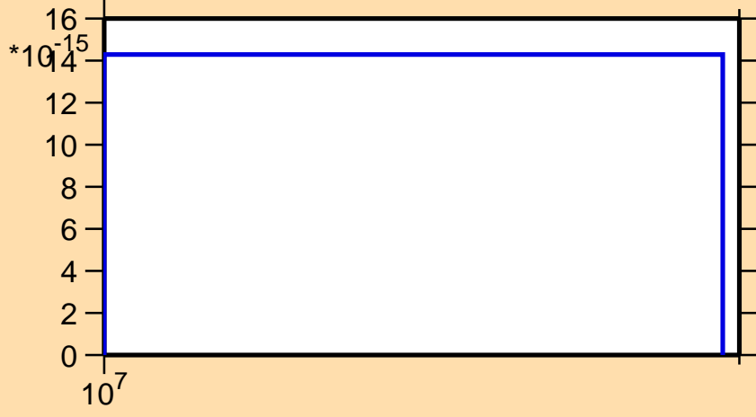
\sigma vs. E for ^{248}\text{Fm} (mt 34)
