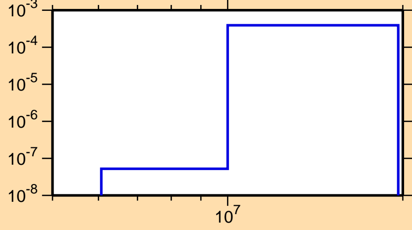
\sigma vs. E for ^{248}\text{Fm}(n,np)
