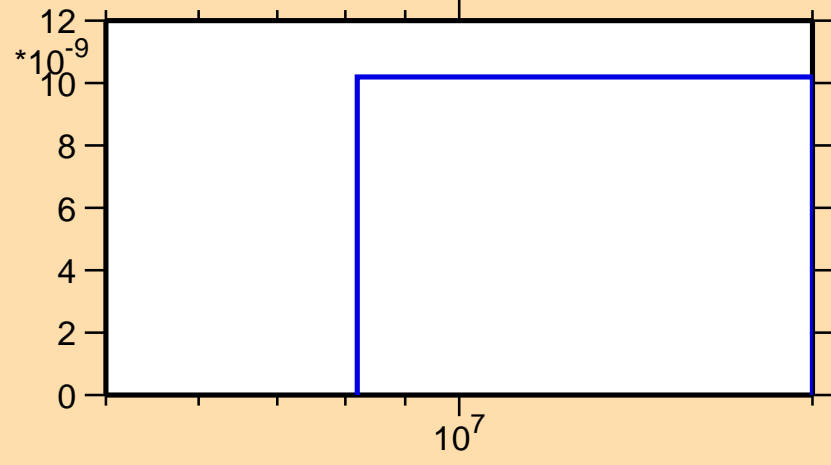
\sigma vs. E for ^{248}\text{Fm}(n,\text{nd})
