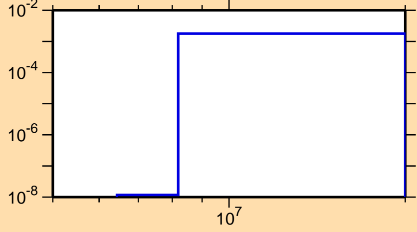
\sigma vs. E for ^{248}\text{Fm}(n,2n\alpha)
