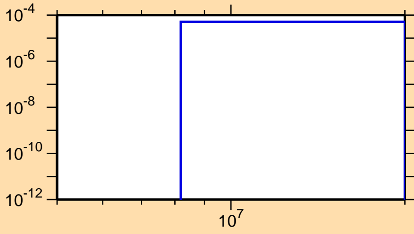
\sigma vs. E for ^{248}\text{Fm}(n,t)
