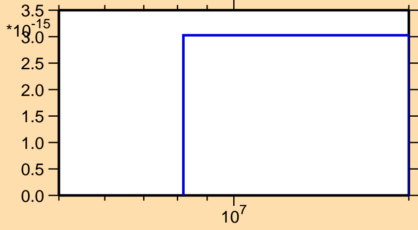
\sigma vs. E for ^{248}\text{Fm}(n,pd)
