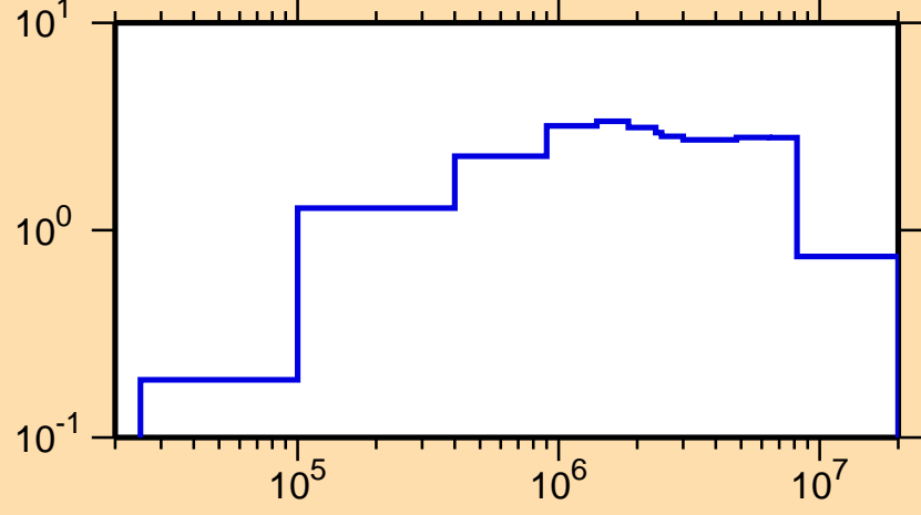
\sigma vs. E for ^{248}\text{Fm}(n,\text{inel.})
