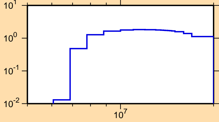
\sigma vs. E for ^{249}\text{Fm}(n,2n)
