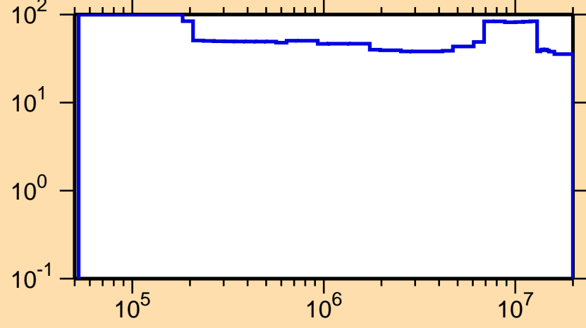
\Delta\sigma/\sigma vs. E for ^{249}\text{Fm}(n,\text{inel.})
