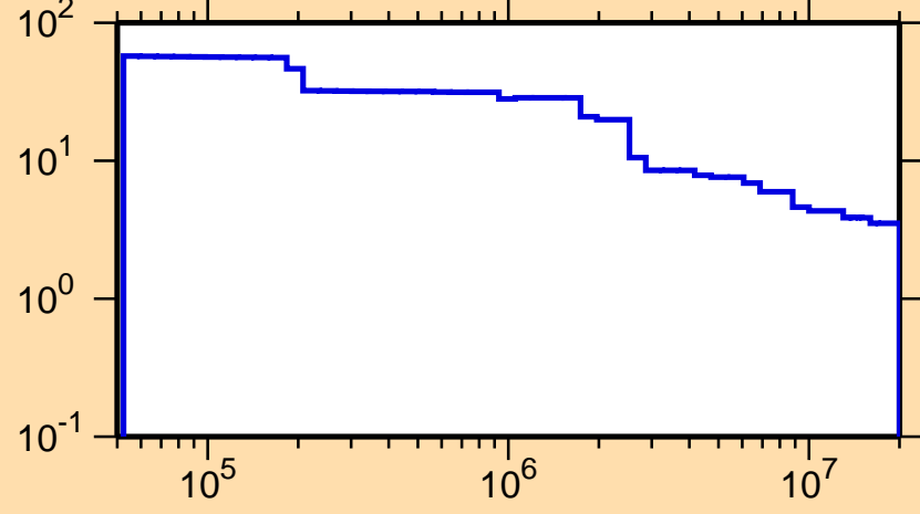
\Delta\sigma/\sigma vs. E for ^{249}\text{Fm}(n,\text{nonel.})
