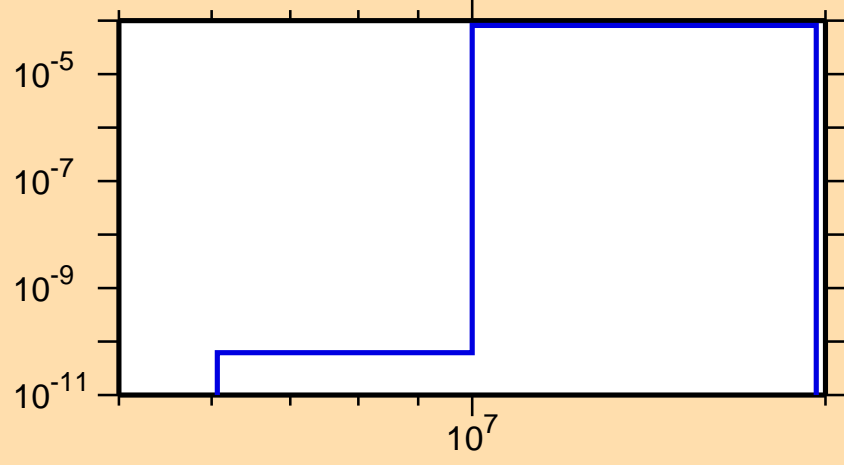
\sigma vs. E for ^{249}\text{Fm}(n,t)
