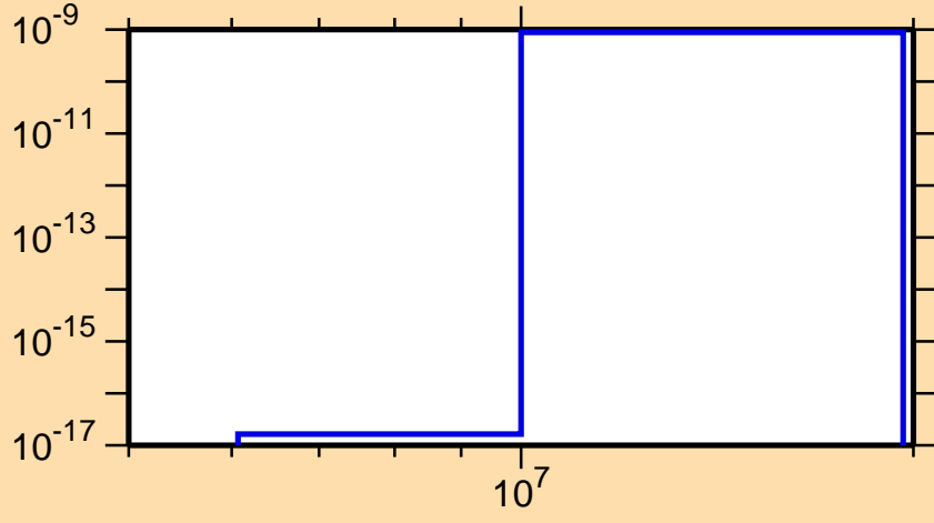
\sigma vs. E for ^{249}\text{Fm}(n,\text{He3})
