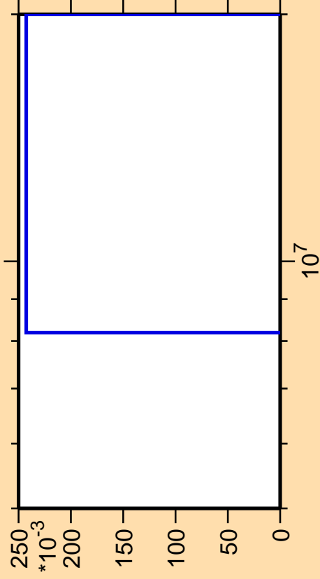
\Delta\sigma/\sigma vs. E for ^{249}\text{Fm} (mt 45)
