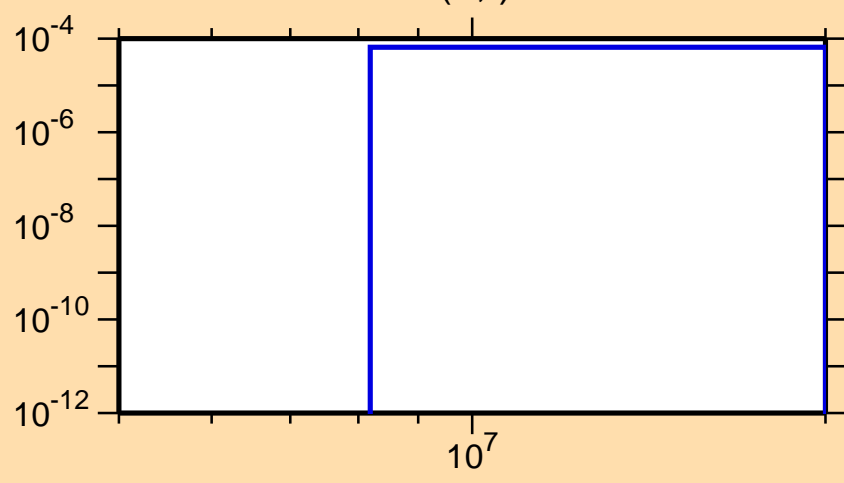
\sigma vs. E for ^{249}\text{Fm}(n,t)
