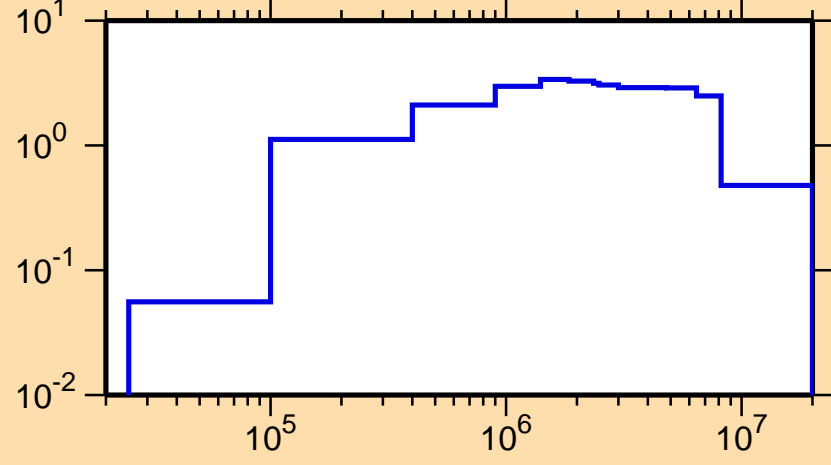
\sigma vs. E for ^{249}\text{Fm}(n,\text{inel.})
