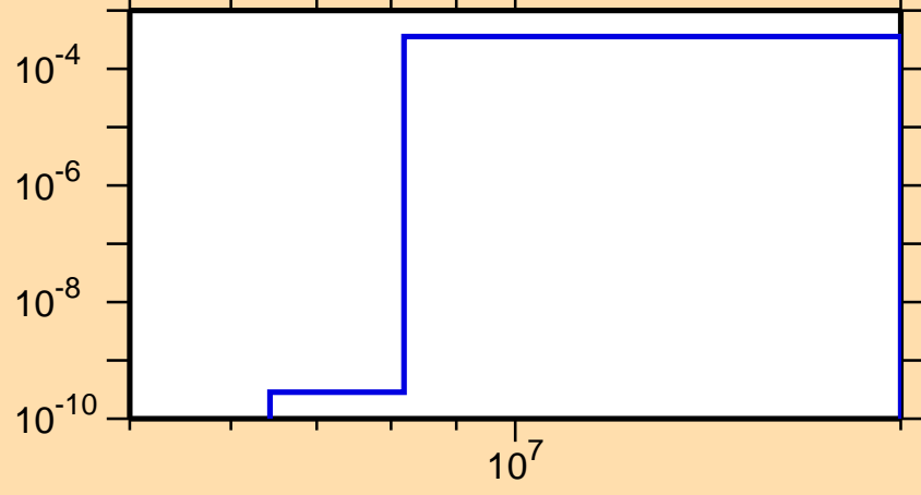
\sigma vs. E for ^{249}\text{Fm}(n,np)
