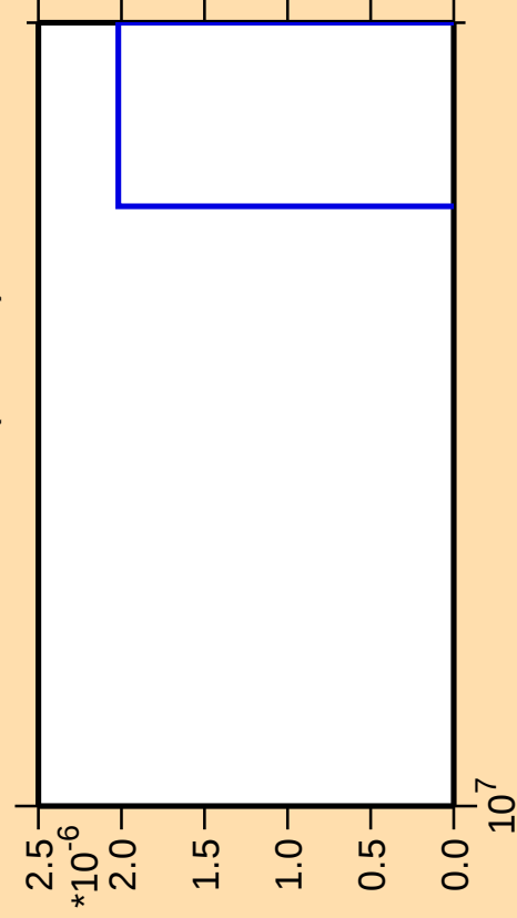
\Delta\sigma/\sigma vs. E for ^{250}\text{Fm}(\text{mt } 42)
